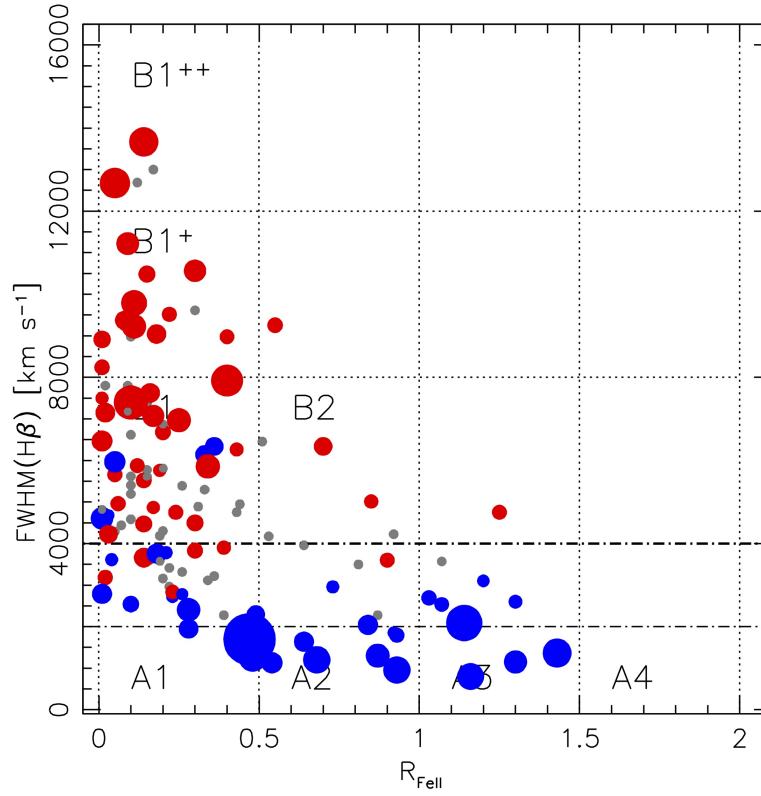
Figure 2. Bias of the M_{\text{BH}} estimates in the optical E1 plane \text{FWHM}(\text{H}\beta) vs. R_{\text{FeII}} , for the full sample of Sulentic et al. [6]. Grey symbols represent differences |\Delta \log M| = |\log M(\text{CIV}) - \log M(\text{H}\beta)| \leq 0.3 , blue dots \Delta \log M > 0.3 , red circles \Delta \log M < -0.3 . The size of the circles is proportional to the amplitude of the difference, with the largest blue circles showing CIV masses in excess by a factor 100. Mid-sized circles indicate a disagreement of a factor \approx 10 . The labels identify the spectral types as described in Section 4 and the thick dot-dashed line at 4000 \text{ km s}^{-1} shows the boundary between Population A and Population B.
