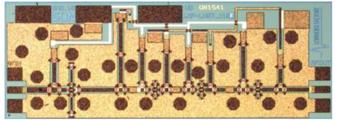
Fig. 22. Photograph of the W-band MMIC LNA from LNF. The die measures 2.0 mm × 0.75 mm.
