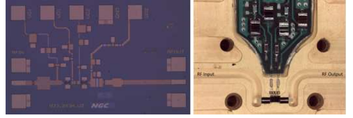
Fig. 21. Left: microscope photograph of one of the fabricated UoM MMICs. The die size of the UoM MMICs is 1.3 mm × 0.9 mm. Right: interior of the packaging showing the MMIC, the waveguide to microstrip transitions, WR10 waveguide channels (with the RF input on the left and output on the right), and the off-chip bias protection circuit. The MMIC die can be seen in the lower middle portion of the photo, below the bias protection circuit. This figure is based on figures presented in Cuadrado-Calle et al. (2017a).
