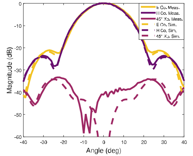
Fig. 12. Upper panel: reflected power S_{11} for the feedhorn designed at INAF. Here, the simulation data are compared with the measurements. The effect of the adaptor used for the measurements is also shown, in lighter purple. Lower panel: INAF feedhorn test results for co-polar (Co) and cross-polar (Xp) beam pattern cuts: E-plane (E), H-plane (H) and 45°-plane. The results for the measurements (lines) versus the simulations (dashed) are shown near the band centre, 91.5 GHz. Our EM simulations confirm that the beam properties scale smoothly as a function of wavelength and, hence, we only show one representative frequency.
