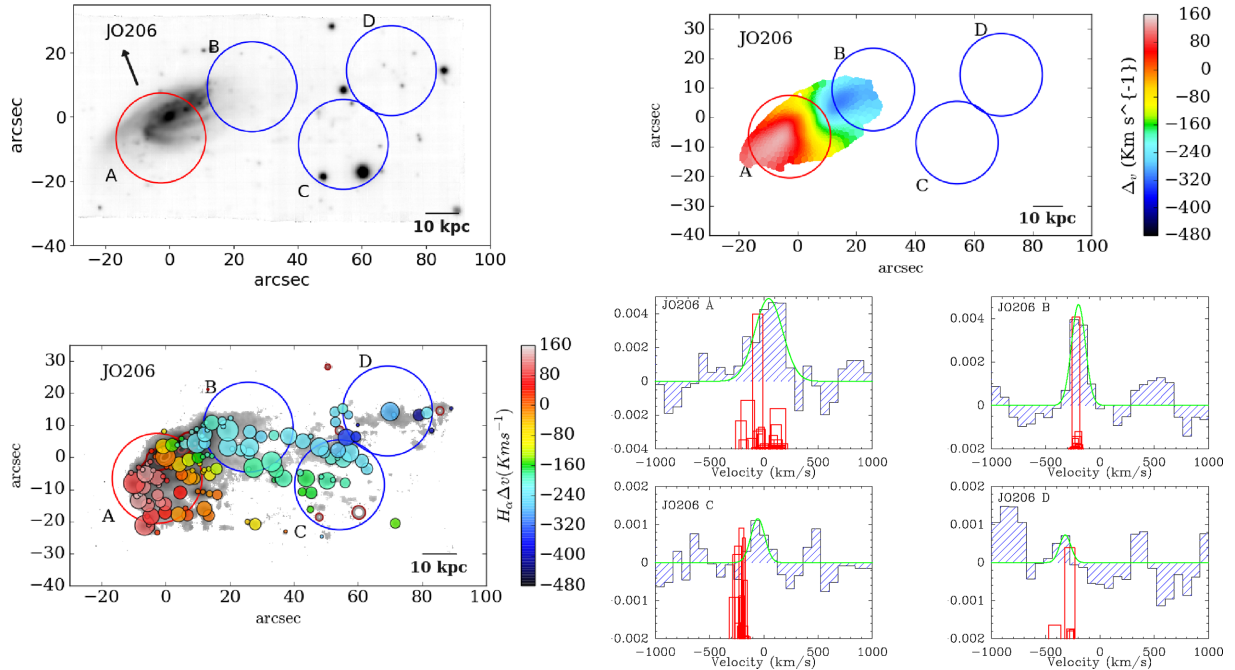
Figure 3. JO206: The upper left-hand panel shows the white light image of the galaxy extracted from the MUSE data cube. The upper right-hand panel shows the stellar kinematics derived from MUSE spectra in Voronoi binned regions with S/N = 10 . The lower left-hand panel shows the galaxy emission determined from the continuum under the H\alpha emission from the MUSE data (in grey) and the star-forming knots colour coded according to their velocity with respect to the galaxy centre. Red (superimposed to the main galaxy body) and blue circles are the observed APEX pointings. The lower right-hand panels show the CO(2-1) spectra ( T_{mb}^* ) in the four positions. In each spectrum, the underlying red boxes correspond to the H\alpha emissions of the star-forming regions within the APEX beam (see text).
