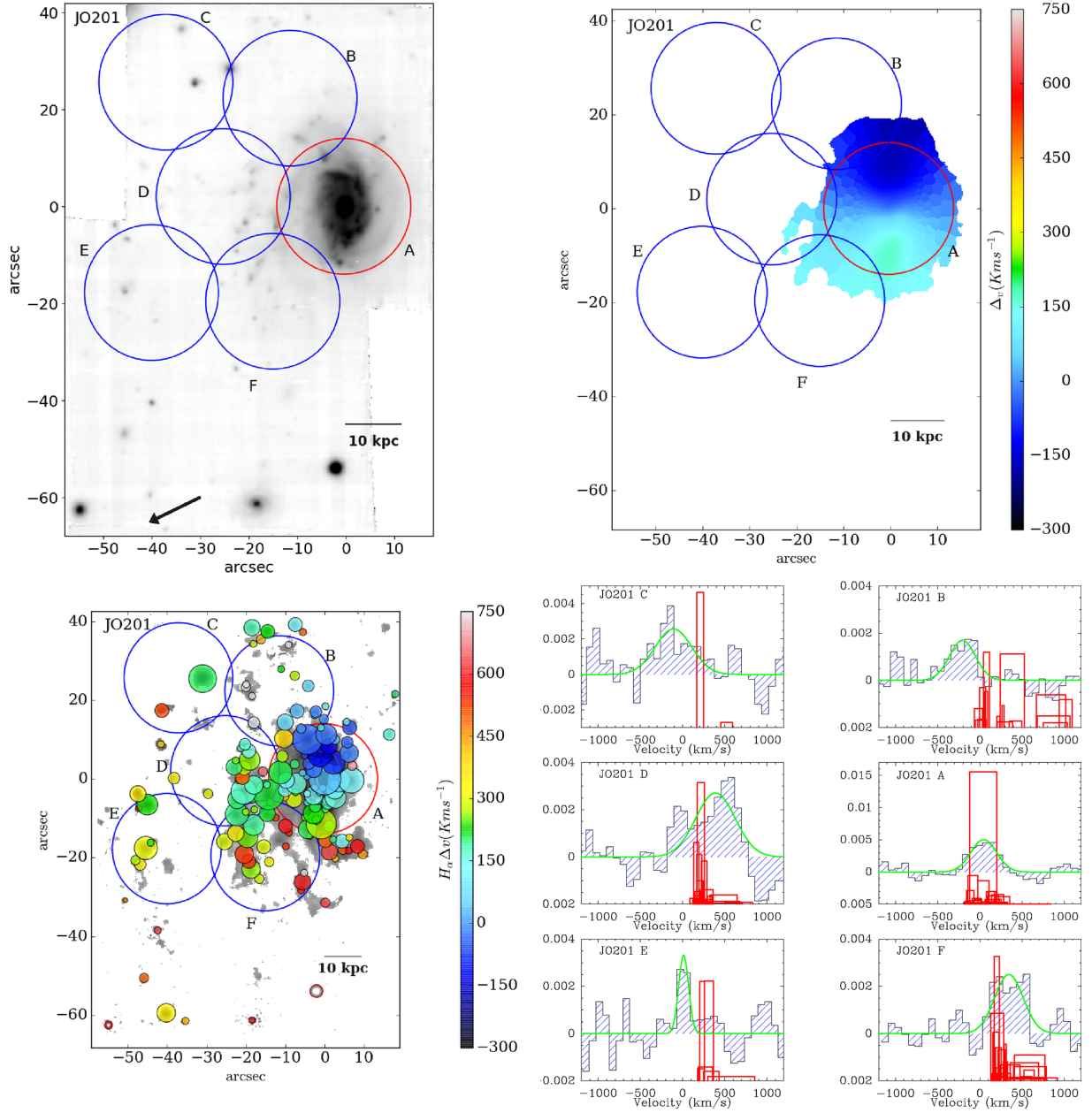
Figure 1. JO201: The upper left-hand panel shows the white light image of the galaxy extracted from the MUSE data cube. The upper right-hand panel shows the stellar kinematics derived from MUSE spectra in Voronoi binned regions with S/N = 10 . The lower left-hand panel shows the galaxy emission determined from the continuum under the H\alpha emission from the MUSE data (in grey) and the star-forming knots colour coded according to their velocity with respect to the galaxy centre. Red (superimposed to the main galaxy body) and blue circles are the observed APEX pointings. The lower right-hand panels show the CO(2-1) spectra ( T_{mb}^* ) in the six positions. In each spectrum, the underlying red boxes correspond to the H\alpha emissions of the star-forming knots within the APEX beam (see text).
