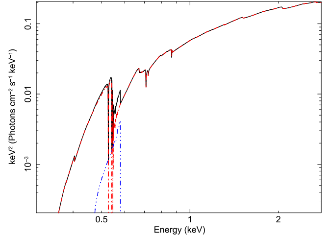
Figure 4. Unfolded model spectrum for XMM-Newton RGS. The blue component corresponds to RELLINE. The red component illustrates RELXILL, which includes the power law.
