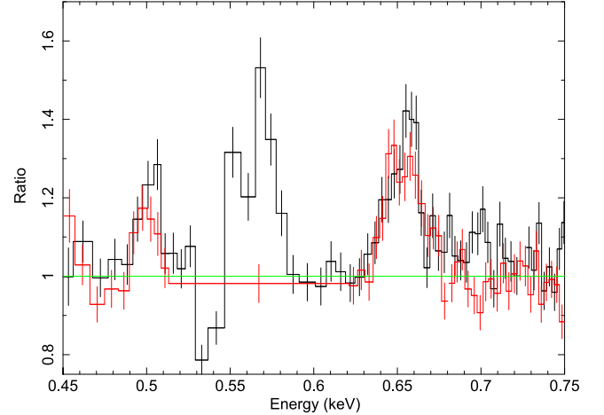
Figure 3. Ratio of the data to the continuum model for XMM-Newton RGS1 (black) and RGS2 (red) showing three emission lines (N VII, O VII, O VIII) and O VIII K edge. The continuum was modeled with a simple absorbed power law that was fit over the energies of 0.45–2.1 keV. The N VII line is located near the edge of the effective area of the detector and therefore not modeled in subsequent fits. The data were rebinned and the x-axis was rescaled for plotting purposes.
