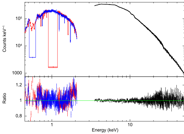
Figure 6. Joint fit of RGS and NuSTAR with TBNEW*(RELXILL+GAUSS+GAUSS+RELLINE) ( \chi^2_{\text{red}} = 1.34 ). The additional RELLINE parameter is needed to model the He-like O VII line. Gaussians were fit at 10.1 and 11.5 keV to account for instrumental response features. The spectrum has been rebinned for plotting purposes. Parameter values can be seen in the fifth column of Table 1.
