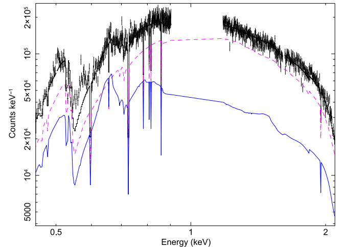
Figure 5. Decomposed RELXILL model spectrum for XMM-Newton RGS1 showing the reflection component (solid blue) and power-law continuum (dashed purple). The RELLINE component is not shown to illustrate the model's ability to fit the O VIII line.
