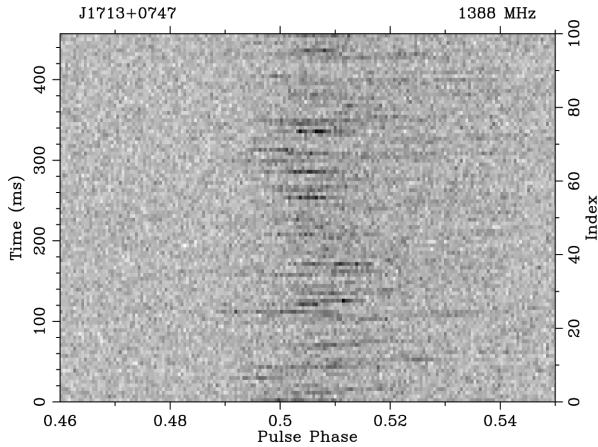
Figure 3. An example of a pulse stack containing 100 pulses. The time resolution used here is 2.3 \mu s. The figure illustrates the pulse-to-pulse variation which is analysed quantitatively further below (see Fig. 7).
