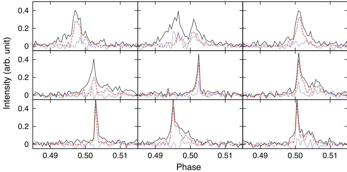
Figure 10. Polarization profiles of the nine highest-S/N pulses. The definition of the lines is the same as in Fig. 2. The time resolution in this plot is 2.3 \mu s.
