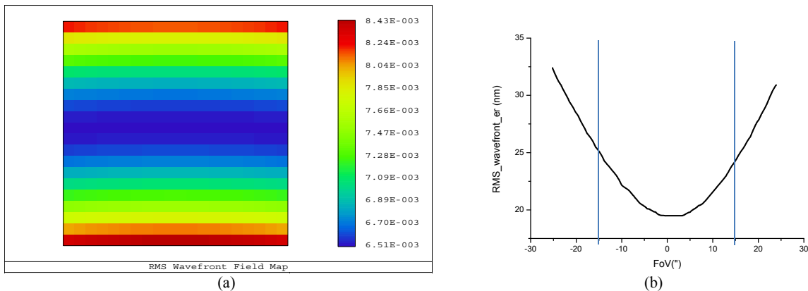
Figure 3. In (a) RMS WFE field map calculated for the 3\ \mu\text{m} wavelength over the 30" nominal telescope FoV. Units are \lambda . In (b) cross section along the Y direction of the RMS WFE expressed in nm; in the X direction the WFE is constant.
