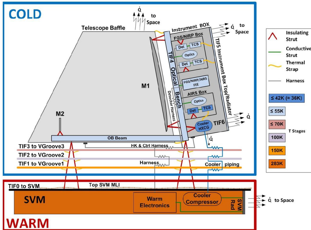
Figure 6. PLM thermal architecture scheme [15].
