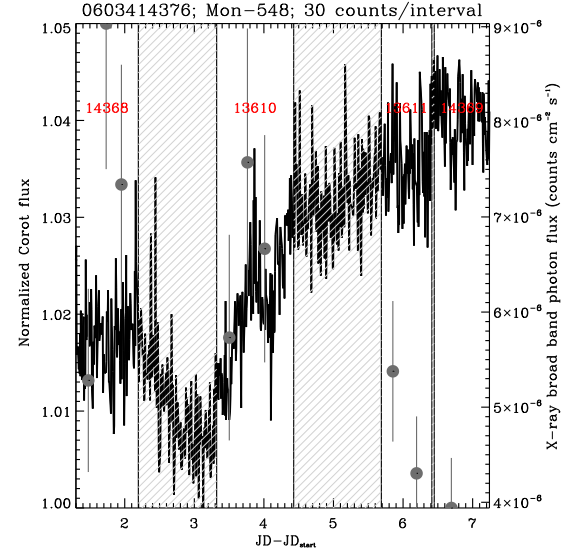
Fig. A.34. Optical and X-ray variability of Mon-548, sorted in the anti-correlated sample. Panel format and content generally follows Fig. 2.
