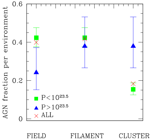
Figure 4. Distribution of radio-selected AGN within different environments for different values of the AGN radio luminosity (expressed in \text{W Hz}^{-1} \text{sr}^{-1} ). Error bars show 1\sigma Poisson uncertainties.
