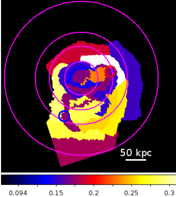
FIG. 4.— Contour binning hardness ratio map of Abell 1142 (2.0–7.0 keV to 0.5–2.0 keV). Blue and red circles indicate the locations of two brightest cluster galaxies. Magenta annuli, centered on the peak of X-ray emission, represent extraction regions of spectral analysis (Figure 3).
