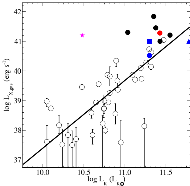
FIG. 11.— Gaseous X-ray luminosities as a function of K -band luminosities for all galaxies taken from Su et al. (2015b). The black solid line is the best-fit L_{X_{\text{gas}}} – L_K relation. Black solid circles indicate group center galaxies. Red circle represents IC664 (G2). Blue symbols represent NGC 3492 (G1)– blue circle: using the average L_{X_{\text{gas}}} and L_K of the three galaxies in G1; blue square: assuming all the L_{X_{\text{gas}}} is from one of the three galaxies; blue triangle: treating all three galaxies as one galaxy (total L_{X_{\text{gas}}} and L_K ). Magenta star represents the small galaxy at the central X-ray peak.
