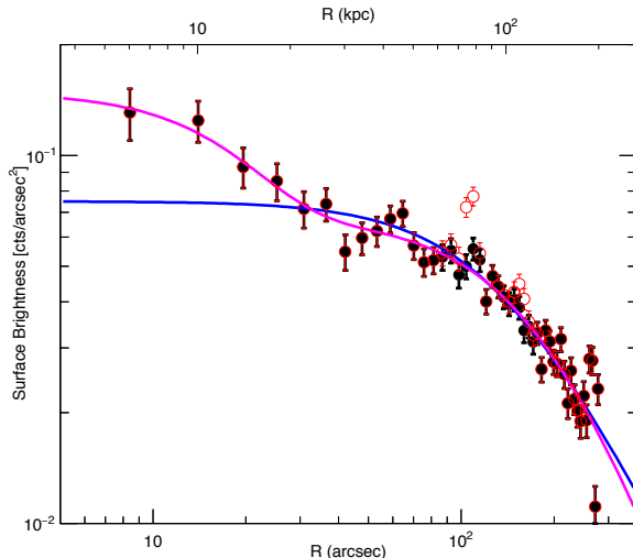
FIG. 2.— Surface brightness profile of Abell 1142 in the energy band of 0.5–4.0 keV, centered on the cluster X-ray emission peak (cyan cross in Figure 1). Blue solid line indicates the best-fit single \beta model with \beta = 0.45 \pm 0.04 and r_c = 92 \pm 16 kpc. Magenta solid line indicates the best-fit double \beta model with \beta = 0.65 \pm 0.13 ( r_{c1} = 12 \pm 4 kpc and r_{c2} = 157 \pm 31 kpc).
