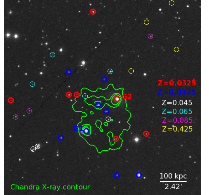
FIG. 5.— . DSS image galaxies of the central 18' × 18' of Abell 1142. Chandra X-ray contour is based on an adaptively smoothed image; contour levels are at [0.9, 1.5, 2.1] \times 10^{-9} photon cm -2 s -1 . We overlaid the redshift distributions of SDSS galaxies (only those with at least three galaxies per redshift bin are shown here).
