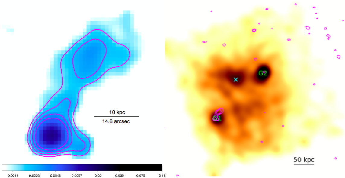
FIG. 10.— . left : VLA radio image of G1 showing extended radio emission in the northwest direction in the unit of \text{Jy beam}^{-1} . Magenta contour levels are set at \sqrt{[1, 2, 4, 8]} \times 4\sigma_{\text{rms}} where \sigma_{\text{rms}} = 0.37 \text{ mJy beam}^{-1} . right : Chandra X-ray image of Abell 1142 with radio contour overlaid.
