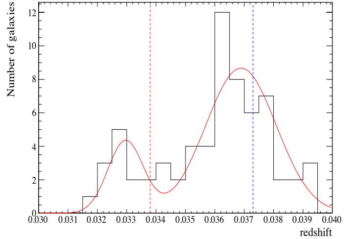
FIG. 8.— Histogram of the redshifts of the final sample of members of A1142 within 1.5 Mpc using a bin size of \Delta z = 0.0005 . Blue and red dashed lines indicate the redshifts of G1 and G2 respectively.
