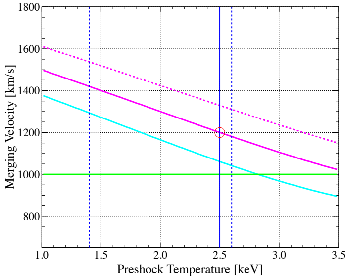
FIG. 12.— Estimated merging velocities between the two subclusters as a function of the ICM preshock temperatures for Abell 1142. Cyan and magenta solid (dashed) lines represent postshock temperatures of 3.5 keV and 4.0 keV (4.5 keV) respectively. Green solid lines indicates 1000 \text{ km s}^{-1} , the radial merging velocities inferred from the redshift distributions of member galaxies. Two blue dashed lines indicate 1.4 keV and 2.6 keV covering the range of preshock temperatures inferred from the cluster L_X and \sigma respectively. We marked a preshock temperature of 2.5 keV in blue line, inferred from the temperature profile of Abell 1142 out to 200 kpc. Red circle indicates the most likely scenario.
