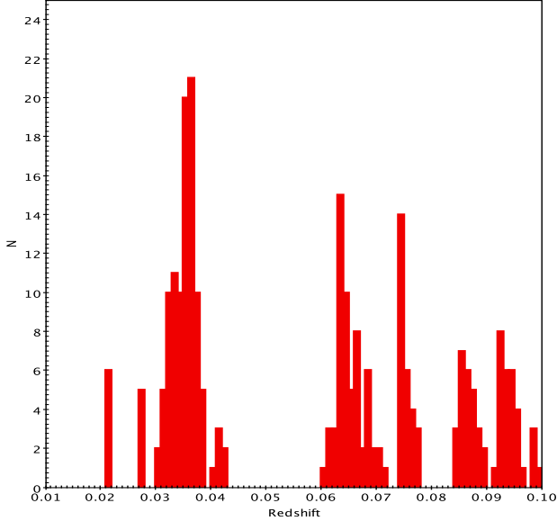
FIG. 6.— Histogram of all the available redshifts in the SDSS database and NED within a 60' field (galaxies with z > 0.1 are not shown for display purposes). The Abell 1142 group stands out as the redshift peak at z = 0.035 .
