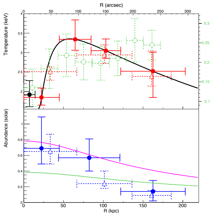
FIG. 3.— Projected temperature (top) and metal abundance (bottom) profiles of Abell 1142 centered on the peak of X-ray emission (four magenta annuli in Figure 4). We also show the results of a different radial binning of three annuli (dashed line). Black solid line is the best-fit temperature profile. We added hardness ratio profile in the top panel (green open circles). Magenta (green) solid line is the average metal abundance profile of CC (NCC) clusters studied in Ettori et al. (2015).
