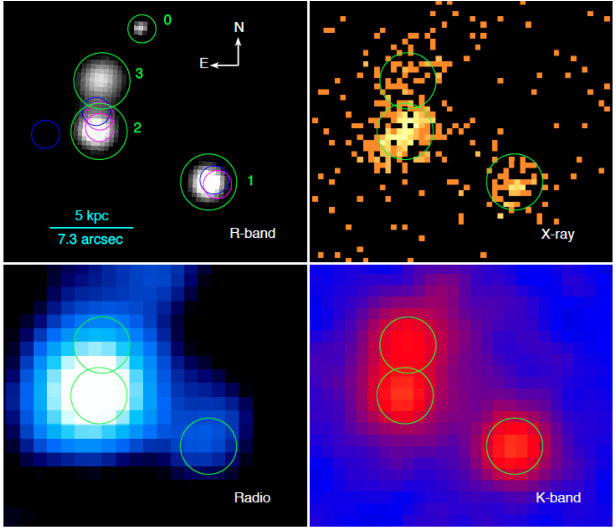
FIG. 9.— . R -band (SDSS), X-ray ( Chandra ), Radio (VLA), and K -band (2MASS) images of G1 (NGC 3492) on the same scale. Objects 1, 2, 3 are early-type galaxies. Object 0 is a foreground star. Magenta circles are positions of three galaxies listed in NED and blue circles are three galaxies listed in HyperLeda.
