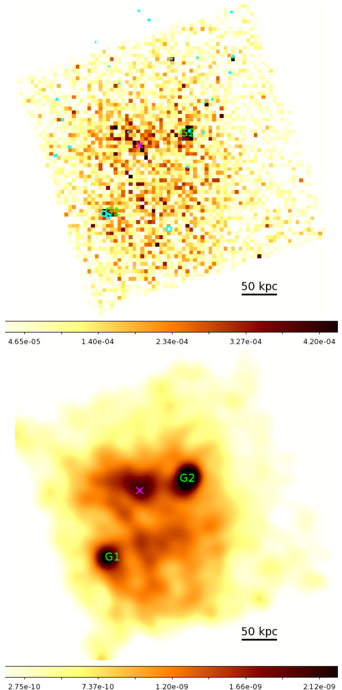
FIG. 1.— 27 ksec exposure-corrected and blank-sky background subtracted Chandra ACIS-S image of Abell 1142 and in the energy band of 0.5–4.0 keV. top : The image was binned by 16 \times 16 pixels in the unit of counts/s. Positions of point sources were marked in cyan ellipses. bottom : adaptively smoothed in the unit of \text{photon cm}^{-2} \text{ s}^{-1} . Locations of G1 and G2 are indicated. The peak of cluster gas emission is indicated by magenta cross.
