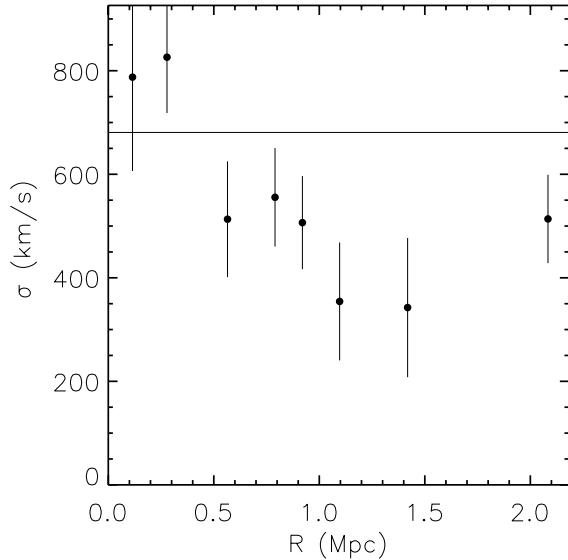
FIG. 7.— Velocity dispersion profile of the Abell 1142 group, where the center of the group is assumed to be at the position of the galaxy IC 664. Bins contain 10 galaxies each and 1\sigma jackknife errors are shown. The solid line shows the expected value of dispersion velocity assuming density-energy equipartition between IGM and galaxies, i.e. \beta_{\text{spec}} = 1 .
