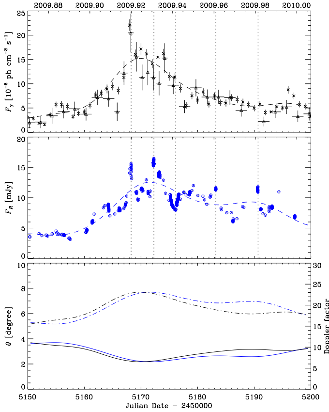
Fig. 8. Flux variations of 3C 454.3 at \gamma -ray (top) and optical (middle) frequencies in late 2009. The \gamma -ray light curve is built with Fermi data (crosses) from Ackermann et al. (2010) and AGILE data (triangles) from Pacciani et al. (2010). Vertical dotted lines indicate remarkable optical events. Cubic spline interpolations through the 7-day binned optical (blue dashed line) and \gamma (black dashed line) light curves are also shown. They represent the variations due to geometrical changes. The evolution of the Doppler factor \delta (dot-dashed lines) and viewing angle \theta (solid lines) is shown in the bottom panel for both the \gamma -ray (black) and optical (blue) bands.
