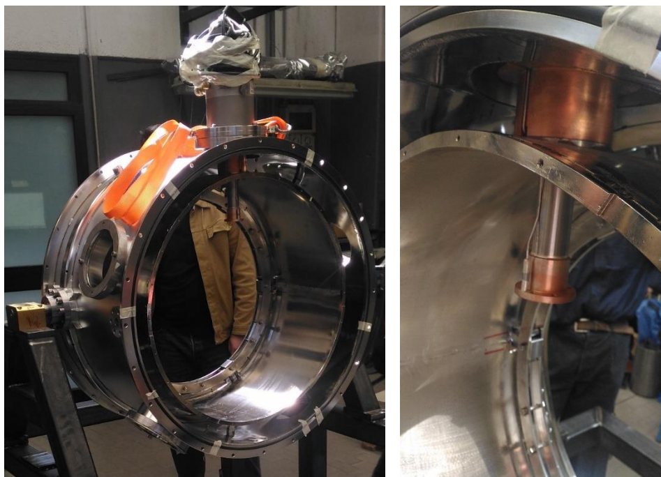
Figure 2 Left panel: a global view of the side surface of the cryostat outer wall and 80 K shield. Right panel: a detailed view of the cooler cold head interfaces.
