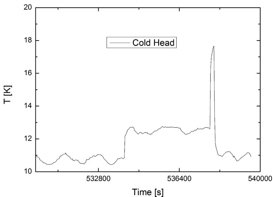
Figure 11 The 20K cold head temperature curve during the heat load test phase.
