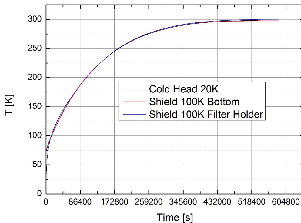
Figure 13 The cryostat warmup temperature curve
