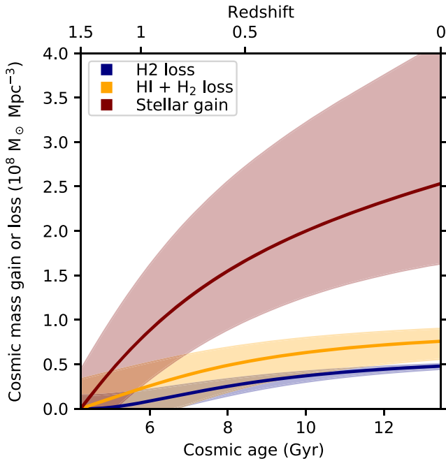
Figure 5. Cumulative gain of the stellar mass density (red line) compared to the cumulative loss of the gas mass density ( H_2 : blue line, total gas: orange line), starting at a redshift of z = 1.5 ( T_{\text{Univ}} \sim 4 Gyr), i.e., approximately the peak of the molecular gas density. The lower (upper) abscissa shows cosmic age (redshift). Even assuming that 100% of the gas will end up in stars, the gas observations cannot account for the observed stellar mass buildup. The remaining mass to build up the stellar mass must be accreted onto the galaxy.
