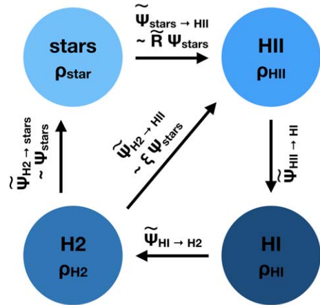
Figure 9. Diagram of the flows between the different main baryonic phases (stars, ionized gas \text{HII} , atomic gas \text{HI} , molecular gas \text{H}_2 ) in the universe. The phase evolution can be expressed with 12 flow rates \psi_{x \rightarrow y} that describe the 4 phases \rho_x as indicated in the left panel (Equations (A1)–(A4)). Darker arrows indicate the main flows in the diagram. The right panel shows how the flows are simplified, by setting some flow terms to zero (see text) and introducing net flows that are marked with a tilde.
