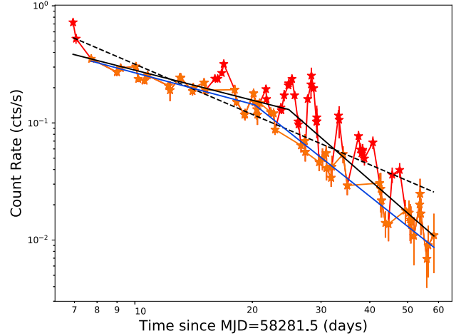
Figure 4. A log–log plot of the XRT light curve indicates that the evolution of the X-ray emission follows a broken PL with a break at day T_d + 21 . Three fits are shown: fitting all data with a single PL (black dashed line), or with a broken PL (black line) as well as a fit to the data excluding obvious flaring points (blue line). The flaring points that are shown here in red.
