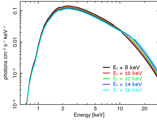
Fig. 7 The HMXB spectral models used in the simulations.
