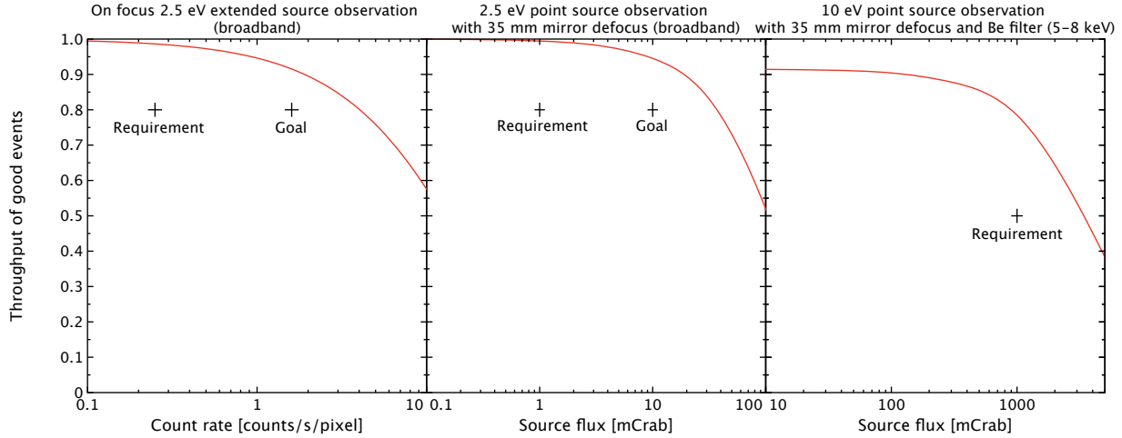
Figure 5. Throughput of good events for the three sizing science cases for the X-IFU count rate capability. Left: High resolution observation of an extended source with a thermal spectrum. Middle: High resolution observation of a bright defocussed Crab-like point source. 10 mCrab corresponds to a count rate of \sim 650 cps over the array with \gtrsim 600 pixels receiving more than 0.6 cps for a maximum of 1.2 cps. Right: 10 eV observation of the same source but with a beryllium filter cutting most of the low energy events. 1 Crab corresponds to \sim 93000 cps over the full matrix with a maximum count rate of \gtrsim 30 cps and \gtrsim 200 pixels receiving more than 15 cps. In all figures, the ‘+’ signs indicate the X-IFU count rate requirements and goals.
