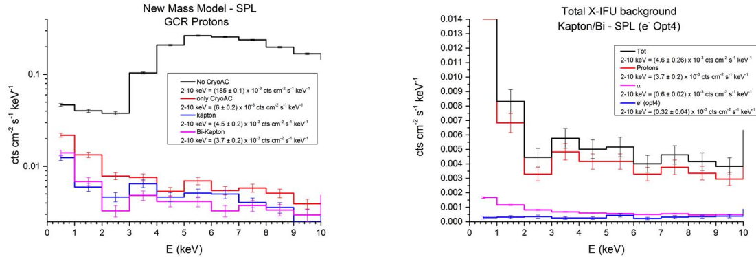
Figure 2. Left: The simulated X-IFU background generated by galactic cosmic ray protons in different configurations: without the CryoAC detector (black line), with the insertion of the CryoAC (red), with a kapton passive shield (blue), and with the optimized kapton/bismuth shield (magenta). Right: Total X-IFU background spectra and integrated values, with all components included (protons, alpha and electrons).
