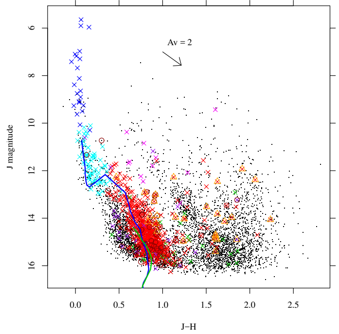
Fig. 16. 2MASS ( J , J-H ) color-magnitude diagram for all IR sources in the ACIS FOV. The blue (green) line is a Siess (BHAC) isochrone at 5 Myr. A representative reddening vector is also shown. Symbols as in Fig. 11. Green crosses are optically unidentified X-ray sources.
