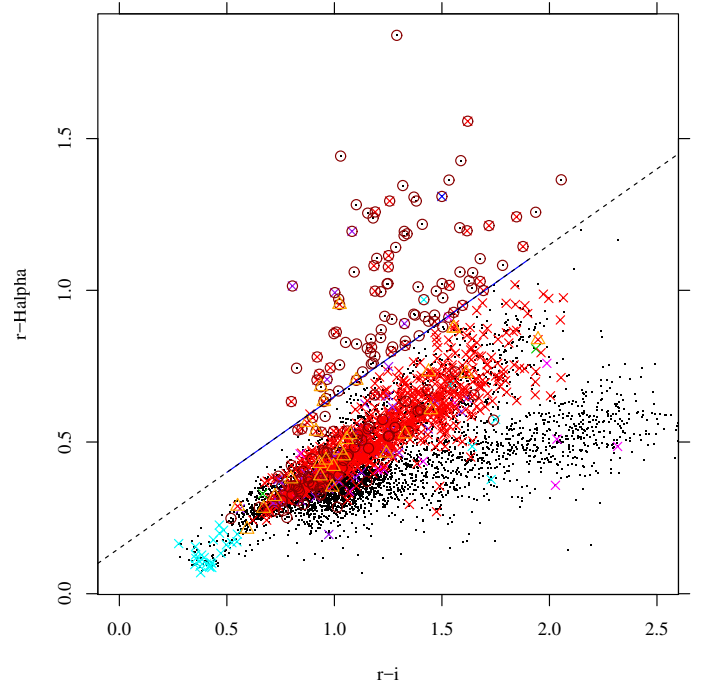
Fig. 12. VPHAS+ index r - H\alpha vs. color r - i . Symbols as in Fig. 11.
