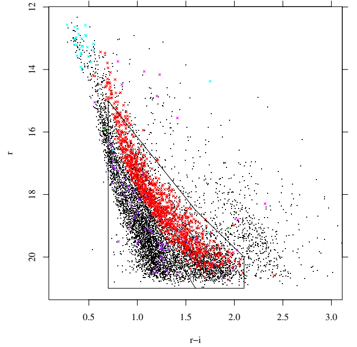
Fig. 6. VPHAS+ (r, r-i) CMD. Symbols as in Fig. 3. The adopted definition of additional VPHAS+ stars in the PMS and Field-MS groups is indicated by the polygons.
