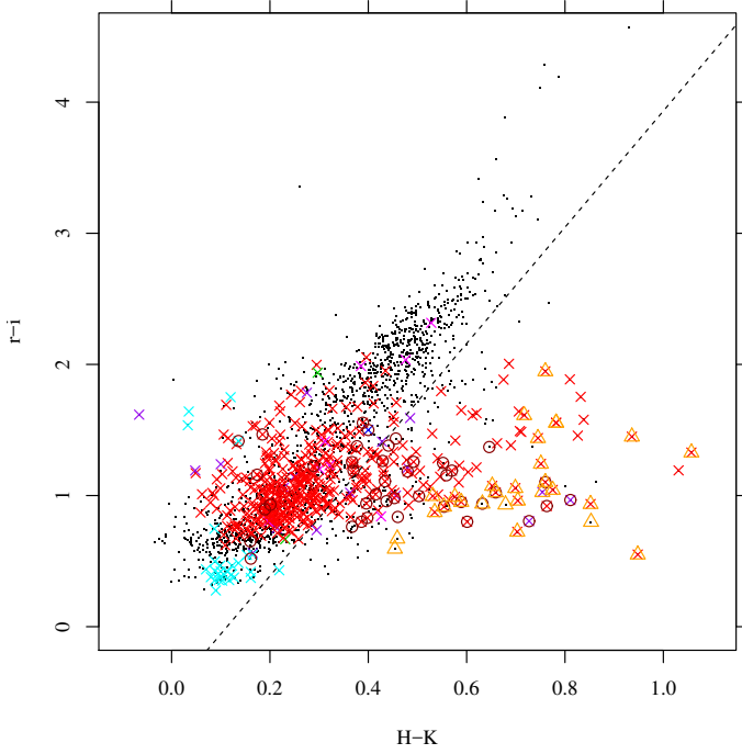
Fig. 15. Optical-IR ( r-i , H-K ) color-color diagram using VPHAS+ colors. Symbols are as in Fig. 4. The dashed line is our adopted limit to select IR-excess stars (orange triangles). Symbols as in Fig. 11.
