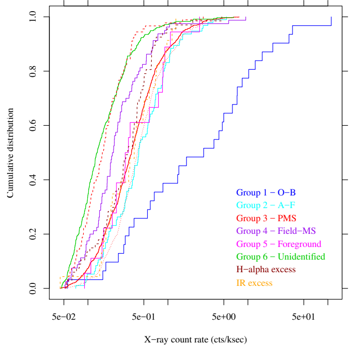
Fig. 29. Cumulative distributions of time-averaged X-ray count rates for the various groups. The PMS group is shown in its entirety (solid red line), and split between stars respectively brighter (dotted red line) and fainter (dashed red line) than V = 20.5 .
