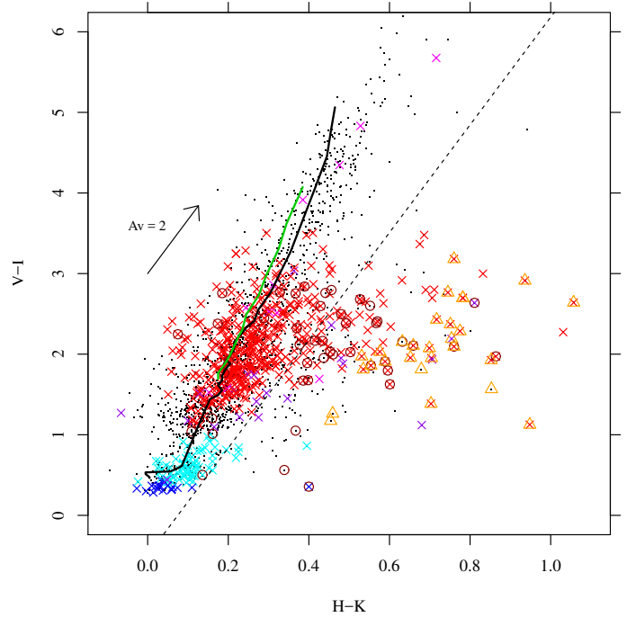
Fig. 14. Mixed optical-IR ( V - I, H - K ) color-color diagram. Symbols are as in Fig. 4. The black (green) solid line is a 5 Myr Siess (BHAC) isochrone for mass M > 0.1 M_{\odot} , the dashed line is our adopted limit to select IR-excess stars. Symbols as in Fig. 11.
