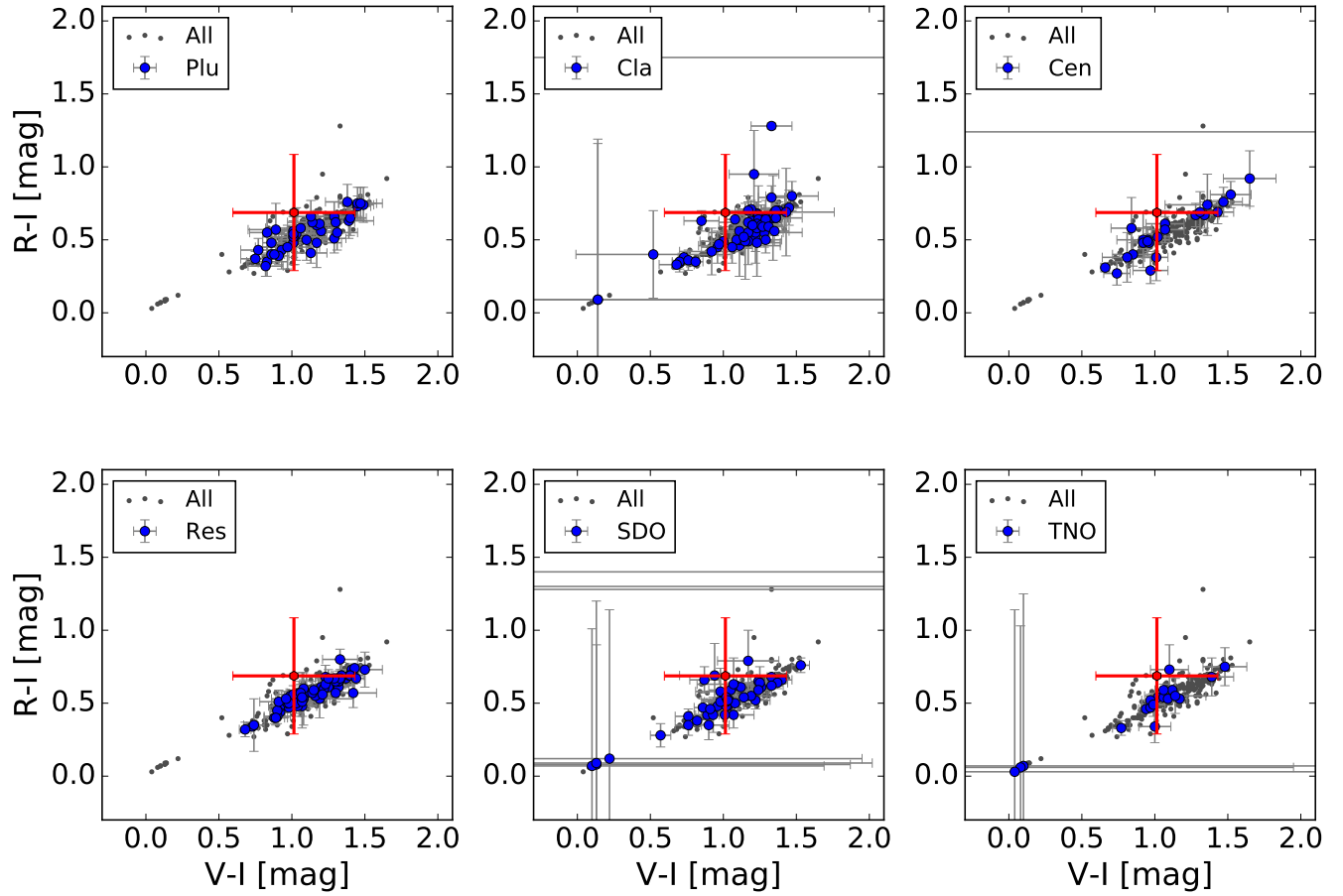
Figure 1. A comparison of the Neso colors from this work with solar system minor body classes from Peixinho, Delsanti, Doressoundiram (2015) . In each frame Neso colors are marked in red and are compared with the colors of a single class from Peixinho, Delsanti, Doressoundiram (2015) represented by blue points, the gray points represents the other classes and are left as a reference. From left to right and from top to bottom: Plutinos (Plu), Classical KBOs (Cla), Centaurs (Cen), Resonant (Res), Scattered Disk Objects (SDO), Trans Neptunian Objects (TNO). All the VRI photometry used to derived the average colors of Neso shown in red are listed in Tab. 1
