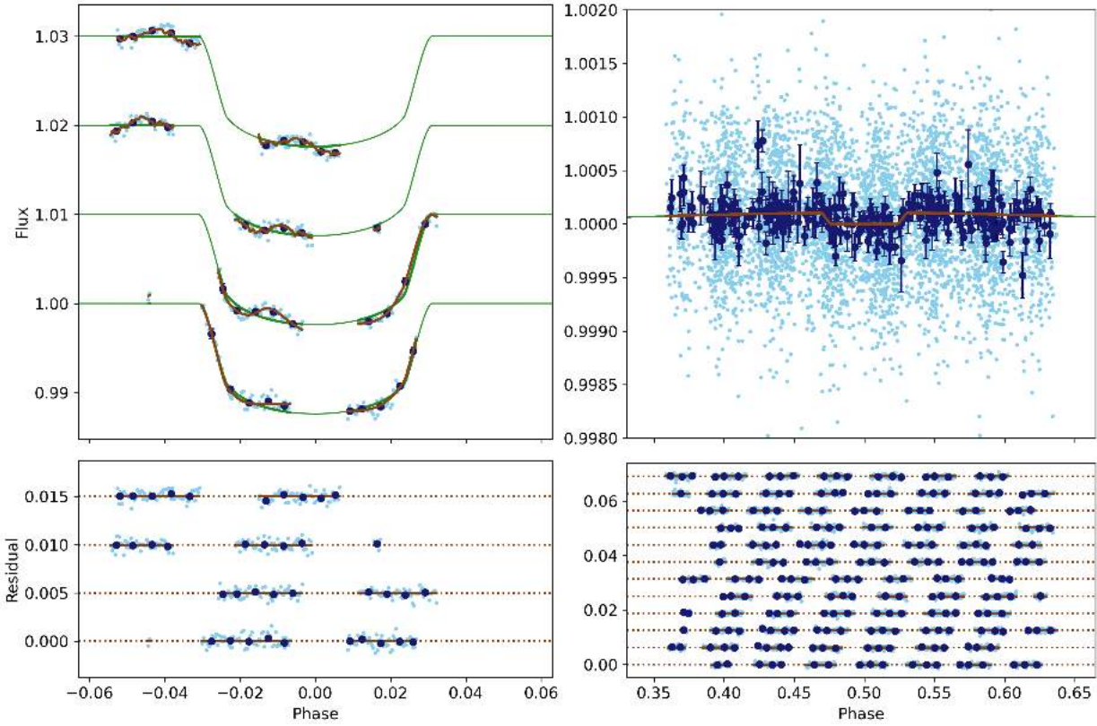
Fig. 3. CHEOPS LC of WASP-3 and our best-fit model for the transits and eclipses. Upper-left panel: observed transit LCs (in cyan) offset vertically by multiples of 0.01 units. The dark blue points are the data points binned over 0.01 phase units. The full model, which includes instrumental trends, is shown in brown, and the transit model without trends is shown in green. Lower-left panel: residuals from the best-fit model to the transit LCs offset vertically by multiples of 0.005 units. Upper-right panel: Secondary eclipse LCs after removal of instrumental noise from our best-fit model, plotted without any vertical offset. Lower-right panel: residuals from the best-fit model to the secondary eclipses offset vertically by multiples of 0.005 units.
