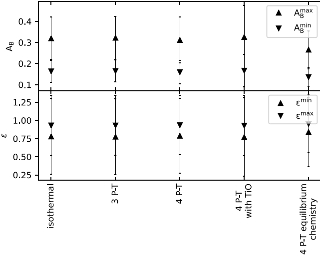
Fig. 10. Maximum and minimum Bond albedo, A_B , of WASP-3 b depending on the assumed thermal model (see the text) and corresponding minimum and maximum recirculation efficiency (top and bottom panel, respectively).
