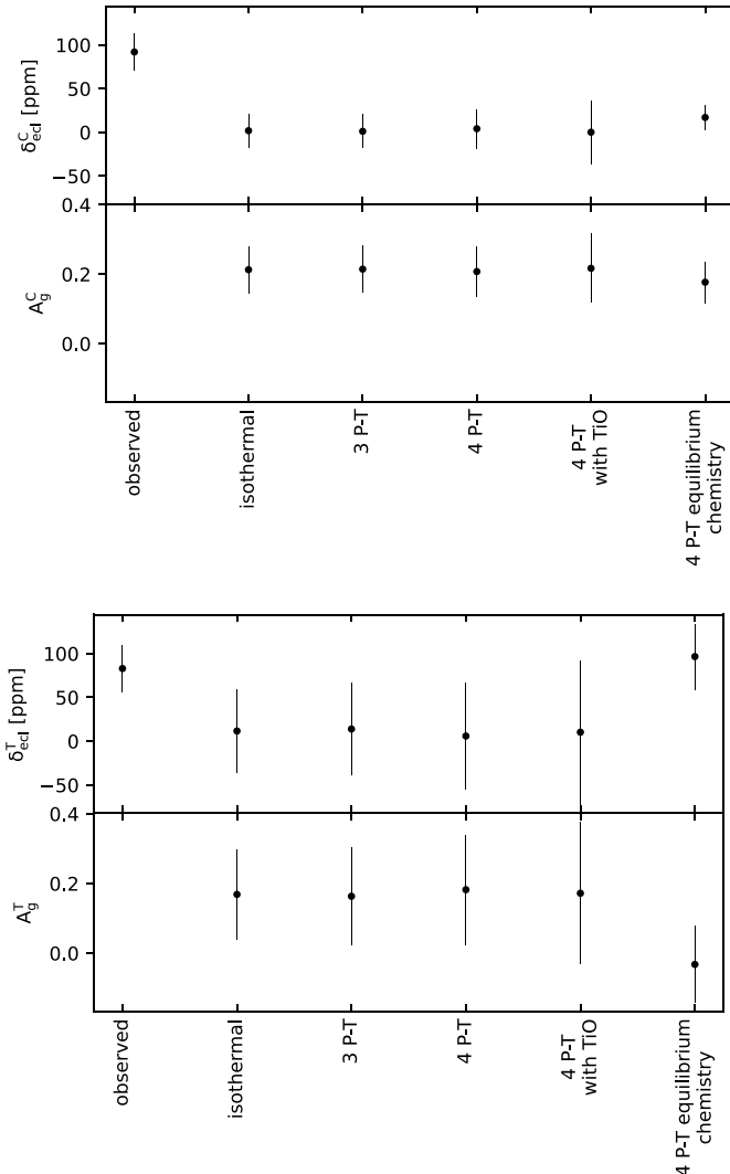
Fig. 8. Measured eclipse depth in the CHEOPS ( \delta_{\text{ecl}}^{\text{C}} , top panel) and TESS ( \delta_{\text{ecl}}^{\text{T}} , bottom panel) passbands together with the theoretical predictions discussed in the text. In each panel, the bottom boxes show the corresponding geometric albedos after correction for thermal emission.
