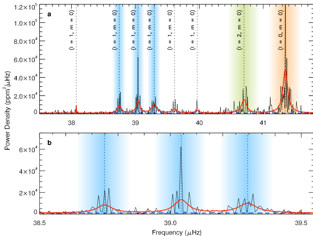
Supplementary Figure 1 | Bayesian peak bagging analysis and fit to the inclination angle. a , A chunk of power spectrum for the core-He-burning red giant KIC 512373 having a low inclination angle. The Bayesian fit to the oscillations 18,19 is indicated by the red line, with the individual mode frequencies marked by a vertical dotted line and the mode identification by labels. The green and orange vertical bands highlight the regions containing the quadrupole ( l = 2 ) and radial ( l = 0 ) modes, respectively. The blue bands indicate the three dipolar mixed modes used to fit the inclination angle of the stellar spin (see Methods). The dashed blue line shows the level of the background signal. b , A close-up in the region containing the three dipolar mixed modes marked by a blue vertical band, with the red line here showing the resulting Bayesian fit to the inclination angle.
