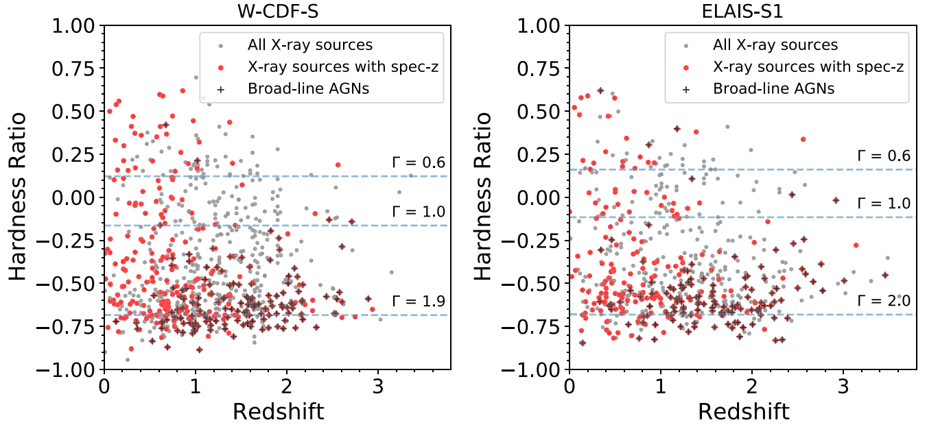
Figure 27. Hardness ratio vs. redshift for X-ray sources that are detected in both the soft and hard bands and have reliable redshift measurements (gray circles) in W-CDF-S (left) and ELAIS-S1 (right). Assuming a power-law spectrum modified by Galactic absorption, effective power-law photon indices can be derived from hardness ratios, which are utilized in AGN selection (objects with \Gamma_{\text{eff}} \leq 1 are classified as AGNs). X-ray sources with spec-z measurements are marked by the red circles; among these sources, BL AGNs are marked as black plus signs.
