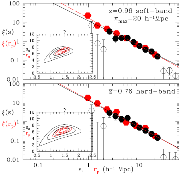
Fig. 5. Redshift-space correlation function, \xi(s) (filled circular points), and the inferred real 3D correlation function, \xi(r_p) (red pentagons), for the soft- (upper panel) and hard-band XXL-S AGNs (lower panel). The black line corresponds to the power-law fit to \xi(s) , and the red line to \xi(r_p) . The empty circular points signify the small and large separation \xi(s) range that are not used in the power-law fit. In the insets we show the 1, 2, and 3\sigma confidence contour levels of the corresponding fitted correlation function parameters.
