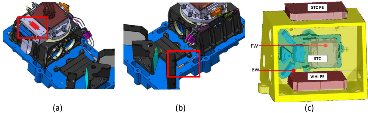
Figure 1 In (a) the location of the “STC Temperature FPA Package (fw)” (NSS21043) temperature sensor (red rectangle). As highlighted in the 3D CAD model (no pictures are available, it is not present in the original CAD model), this sensor is placed onto the FPA package, in the same position where the corresponding sensor is placed on the HRIC FPA. In (b) the location of the “STC Temperature Optical Bench (bw)” (NSS21044) temperature sensor, as shown in the 3D CAD model (no picture available). In (c) the overview of the layout of SIMBIO-SYS showing VIHI and STC PE respect the Temperatures sensors.
