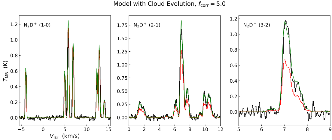
Fig. 10. Red curves show the best-fit model for \text{N}_2\text{D}^+ lines obtained with the fiducial model with initial cloud evolution and \zeta_2 = 1.3 \times 10^{-17} \text{ s}^{-1} , at t = 10^6 yr, overlaid to the observations (black). The used f_{\text{corr}} value is indicated at the top. The modelled lines produced using model \mathcal{F} with no cloud evolution at t = 10^6 yr (and f_{\text{corr}} = 5 ) are shown in green. It is clear that the model with cloud evolution underestimates the (2-1) and (3-2) lines.
