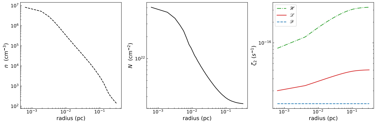
Fig. 1. Left panel: \text{H}_2 volume density profile ( n ) in the physical model of L1544. Central panel: column density profile. Right panel: The \zeta_2 profiles for the \mathcal{F} (dashed blue curve), \mathcal{L} (solid red), and \mathcal{H} (dashed-dotted green) models. The profiles for the models \mathcal{L} and \mathcal{H} P18 have been derived integrating the volume density profile of the core model to obtain the column density profile, and then using the relation between \zeta_2 and N .
