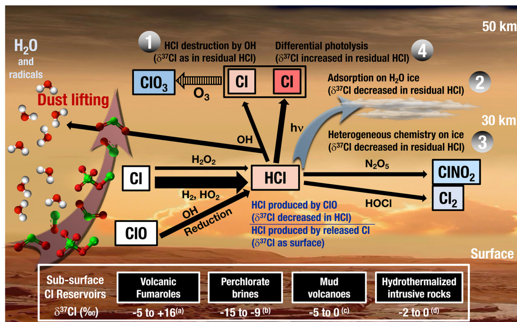
Figure 3. Proposed HCl physics and chemistry and relation with the Cl isotopic composition and reservoirs. Once produced, HCl is then either deposited after photo- or chemical dissociation or processing through heterogeneous chemistry (involving HOCl, \text{N}_2\text{O}_5 ) or adsorption on water ice. The more efficient processes (under Martian conditions) have thicker arrows; the chemistry of \text{O}_3 (dashed arrow) is likely not active at the observations' time. Products with the same isotopic composition as the possible surface reservoirs are in white boxes, those that could be depleted in ^{37}\text{Cl} compared to sources are in red boxes, and those enriched in ^{37}\text{Cl} are in blue. References: (a) Sharp et al. (2010); (b) Böhlke et al. (2005); (c) Godon et al. (2004); (d) Barnes & Cisneros (2012).
