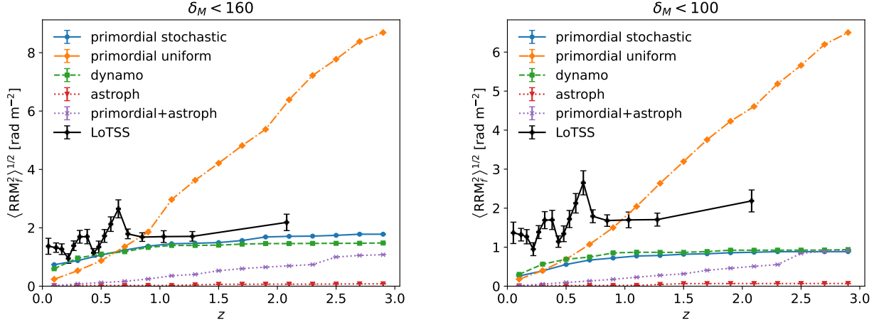
Figure 6. \text{RRM}_f rms in redshift bins computed using density and magnetic field from simulations, for the magnetogenesis models we considered. Two cases differing by the overdensity limit are shown: \delta_M < 160 (left) and \delta_M < 100 (right). The RRM rms from the LoTSS RM catalogue measured in 60-source redshift bins is also shown, with the term A_{rrm}(1+z)^{-2} subtracted off.
