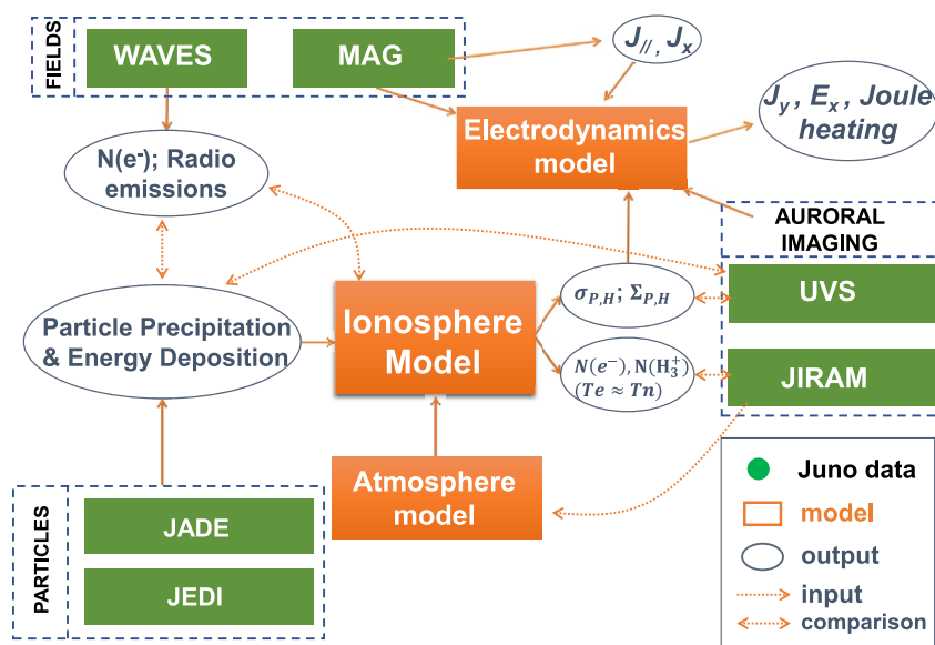
Figure 4. Schematic of the method used to retrieve the key parameters of Magnetosphere-Ionosphere-Thermosphere coupling from Juno data (green boxes) and modeling tools (orange boxes). Using the electron precipitation data obtained from the Juno JADE and JEDI measurements, some of the ionospheric parameters such as conductivities and electron/ion densities can be calculated from the ionosphere model. The electrodynamics model along with the Juno WAVES and MAG data can be used to evaluate the ionospheric currents and Joule heating. The auroral imaging data provide information on the electron precipitations and atmospheric heating, which can be used as a comparison with the results obtained using our method.
