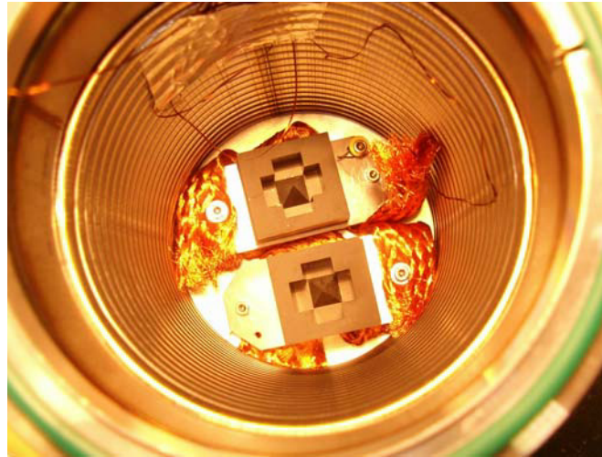
Fig. 1 The two samples imounted inside the dedicated cryochamber.
