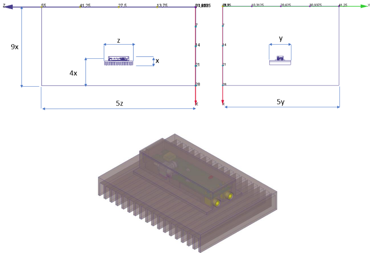
Figure 31 - Optimized case + HS CFD Model
