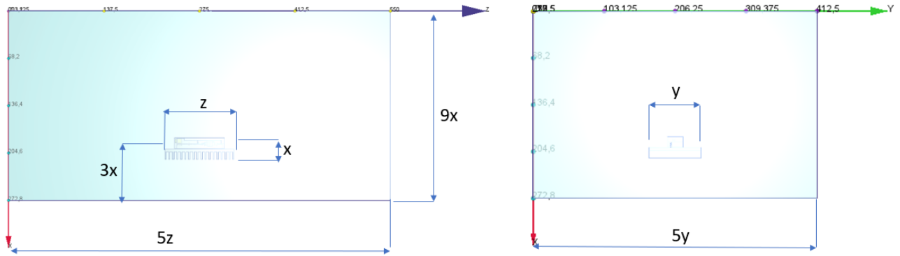
Figure 22 - TX Module +HS CFD model
