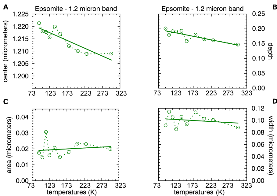
Fig.13. Band parameters determined for the band at 1.2 \mu\text{m} , epsomite. Green circles: 125-150 \mu\text{m} .
