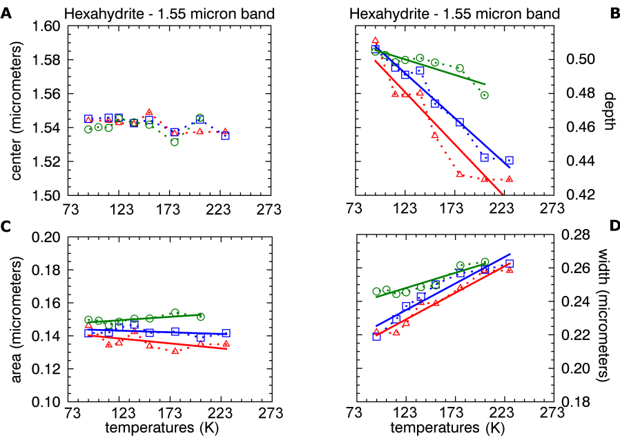
339 Fig.8. Band parameters determined for the band at 1.55 μm, hexahydrite. Red triangles: grain size 20-50 340 μm. Blue squares: 75-100 μm. Green circles: 125-150 μm.
