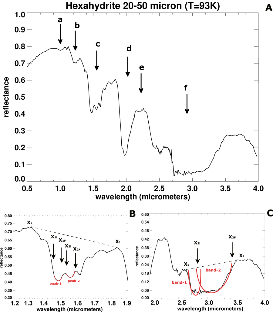
Fig.4. A: absorption bands analyzed in the spectra of the two samples. Band a: 1 \mu\text{m} . Band b: 1.2 \mu\text{m} . Band c: 1.5 \mu\text{m} . Band d: 2 \mu\text{m} . Band e: 2.2 \mu\text{m} . Band f: 3 \mu\text{m} . B: method of band fitting for multi-peak bands. In the case of the broad 1.5- \mu\text{m} feature, the continuum baseline has been drawn between the points X_1 , X_2 . After continuum removal by division, the two minima at 1.47 (peak-1) and 1.55 \mu\text{m} (peak-2) have been fitted with 2 nd order polynomials between two extremes X_{1i} - X_{1F} and X_{2i} - X_{2F} , respectively. Bands have been resampled with 10 3 points before polynomial fitting. The area is computed between X_1 - X_2 and so refers to the area of whole band. C: fitting of the 3- \mu\text{m} band. The edges X_1 , X_2 for continuum removal have been put at 2.6 and 3.54 \mu\text{m} , while the 2 nd order polynomial has been computed, after a denser resampling, between X_{2i} , X_{2F} = 3, 3.42 \mu\text{m} . Band edges X_1 , X_2 and X_{2i} , X_{2F} have been chosen appropriately for each analyzed band and each spectrum, and not kept constant for all dataset, in order to take into account variations from one spectrum to another (i.e. variations with temperature and grain size).
