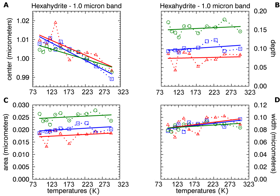
326 Fig.5. Band parameters determined for the band at 1.0 μm, hexahydrite. Red triangles: grain size 20-50 μm. 327 Blue squares: 75-100 μm. Green circles: 125-150 μm.
