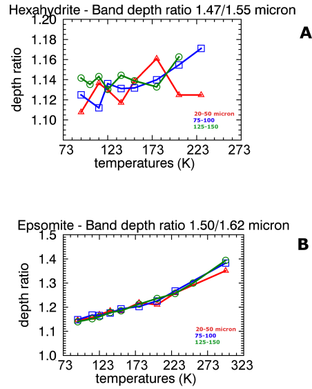
Fig.20. A: depth ratio for the bands at 1.47 and 1.55 \mu\text{m} (hexahydrate). B: depth ratio for the bands at 1.50 and 1.62 \mu\text{m} (epsomite).
