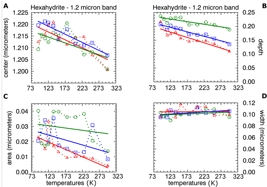
330 Fig.6. Band parameters determined for the band at 1.2 μm, hexahydrite. Red triangles: grain size 20-50 μm. 331 Blue squares: 75-100 μm. Green circles: 125-150 μm.
