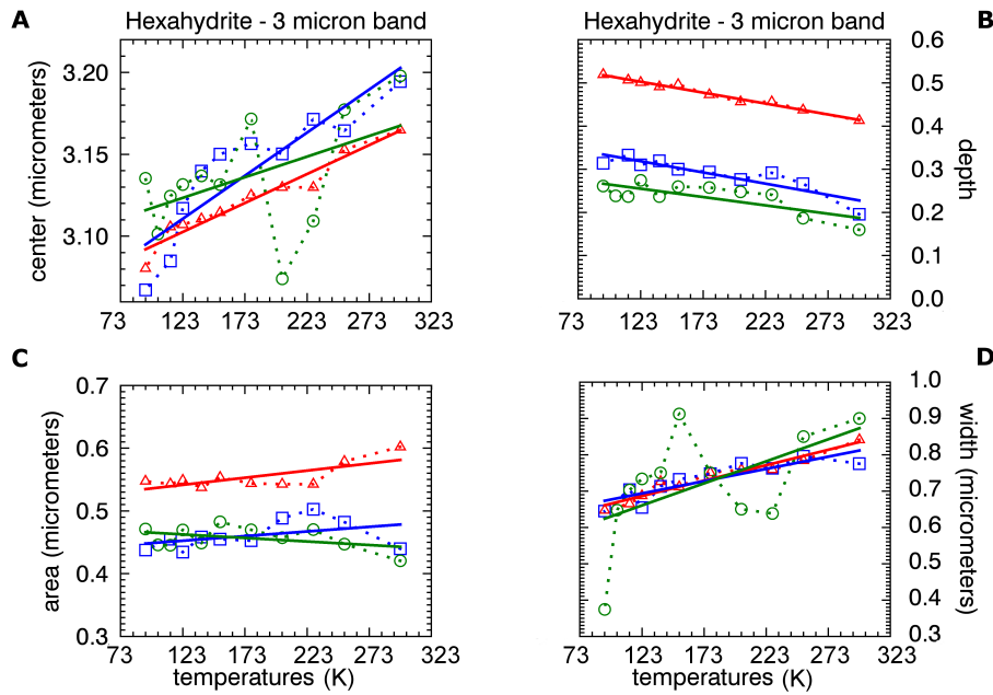
Fig.11. Band parameters determined for the band at 3 \mu\text{m} , hexahydrate. Red triangles: grain size 20-50 \mu\text{m} . Blue squares: 75-100 \mu\text{m} . Green circles: 125-150 \mu\text{m} .
