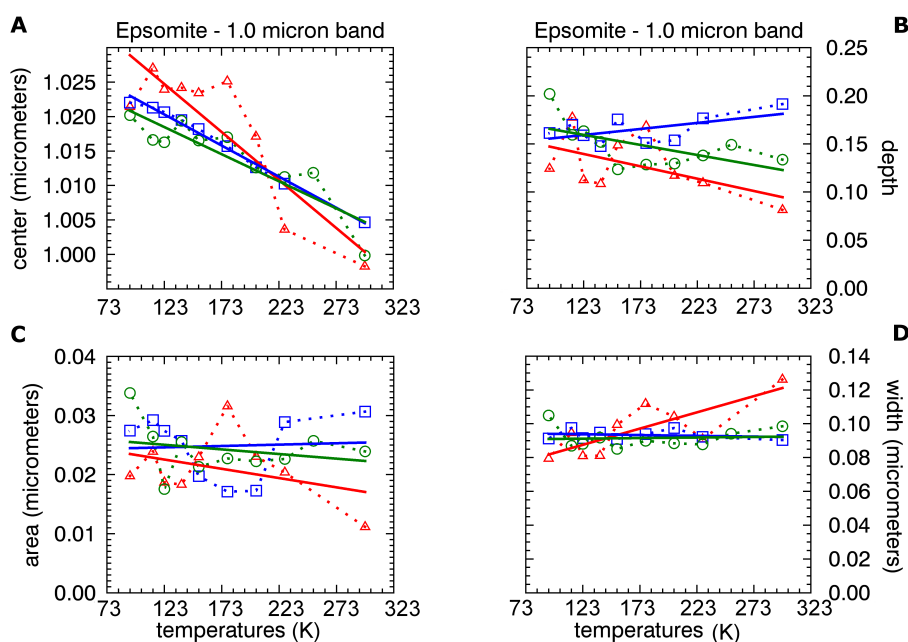
Fig.12. Band parameters determined for the band at 1.0 \mu\text{m} , epsomite. Red triangles: grain size 20-50 \mu\text{m} . Blue squares: 75-100 \mu\text{m} . Green circles: 125-150 \mu\text{m} .
