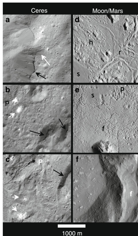
Fig. 2 Floor textures at Occator and large lunar and martian craters.
