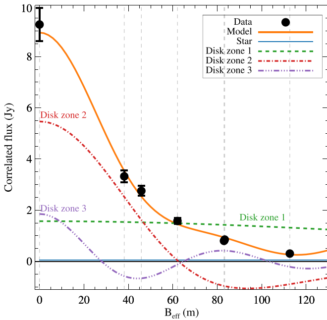
Fig. 2. Correlated flux density as function of the baseline length at a selected wavelength, 10 μm. The contributions of the three disk zones are the green, red, and purple lines, while the correlated flux curve of the whole disk is the orange solid line. Filled circles indicate the MATISSE N -band data points. The zero baseline data point is the single-dish flux. The thin blue line is the contribution of the central star.
