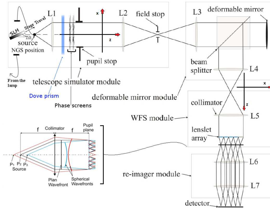
Fig. 1. The concept of LGS Prototype. The images moves in the sub-apertures due to source position along the optical axis (z). The central sub-aperture does not detect a perspective elongation but just a small blur.
