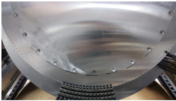
Figure 8. On the left: the aluminium fieldplate on the tumbler as seen from above, with a few empty retractors on the side. On the right: a close-up of the grid machined into the fieldplate. Each point is 0.5 mm wide, and the ones visible here are filled with black paint and lightly sanded.
