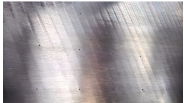
Figure 8. On the left: the aluminium fieldplate on the tumbler as seen from above, with a few empty retractors on the side. On the right: a close-up of the grid machined into the fieldplate. Each point is 0.5 mm wide, and the ones visible here are filled with black paint and lightly sanded.
