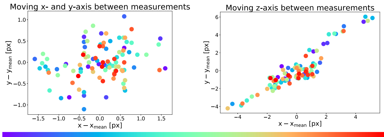
Figure 7. Effect of moving the gripper optical system away from and back to a stationary reference point, 100 data points each. On the left: movement in the x- and y-direction. On the right: movement in the z-direction. The colours denote a time series to check for temporal effects, with blue the early measurements and red the later ones.
