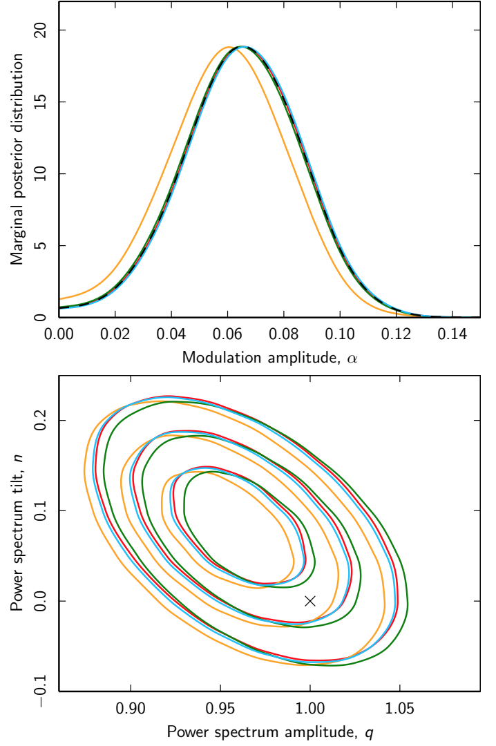
Fig. 29. Top: Marginal constraints on the dipole modulation amplitude, as derived from Planck 2015 temperature observations at a smoothing scale of 5^\circ FWHM for Commander (red), NILC (orange), SEVEM (green), and SMICA (blue). The plot corresponds directly to Fig. 32 of Planck Collaboration XXIII (2014). The Commander , SEVEM , and SMICA posteriors coincide almost perfectly both internally, and with the corresponding SMICA 2013 posterior, shown as a dashed black line. Bottom: Corresponding marginal two-dimensional constraints on the low- \ell power spectrum amplitude and tilt, ( q, n ), defined relative to the best-fit Planck 2015 \Lambda CDM model.
