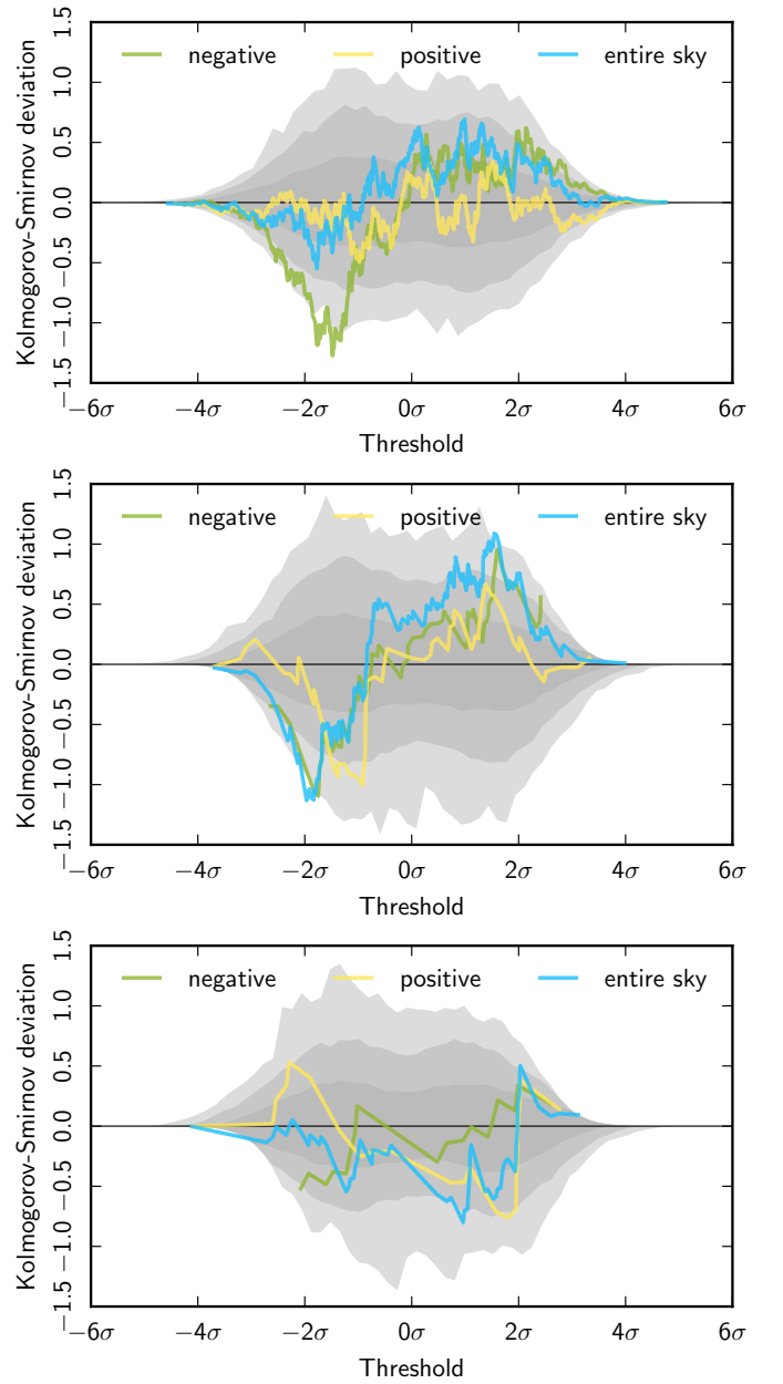
Fig. 22. KS-deviation of the peak distribution for 70^\circ radius discs centred on the positive and negative asymmetry directions determined from the SMICA CMB temperature map in Sect. 6.2. From top to bottom, the plots correspond to maps filtered with a GAUSS kernel of 40' FWHM, an SSG84 filter of 500' FWHM, and an SSG84 filter of 800' FWHM, respectively.
