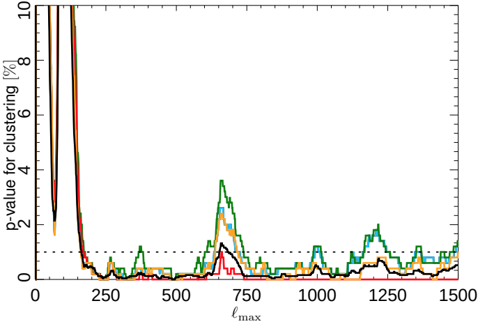
Fig. 36. Derived p -values for the angular clustering of the power distribution as a function of \ell_{\text{max}} , determined for Commander (red), NILC (orange), SEVEM (green), and SMICA (blue), based on 500 simulations. For SMICA, the p -values based on 2500 simulations are also shown (black). The p -values are based on the fraction of simulations with a higher RS, determined over the \ell -range up to the given \ell_{\text{max}} , compared to the data. The results shown here have been marginalized over bin sizes in the range \Delta\ell = 8 to \Delta\ell = 32 .
