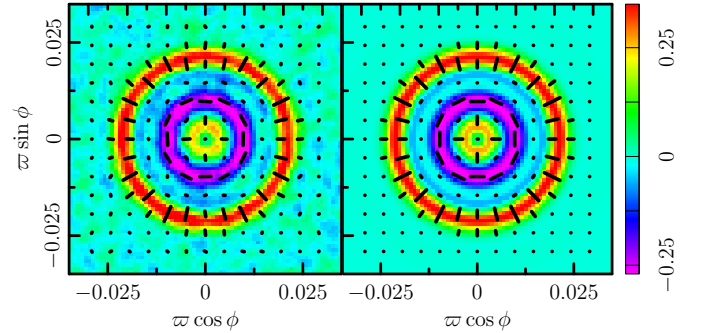
Fig. 46. Stacked Q_r image around temperature hot spots selected above the null threshold ( \nu = 0 ) in the SMICA sky map. The left panel corresponds to the observed data and the right panel shows the NFEA. The image units are \mu\text{K} . The headless vectors (black solid lines) are the polarization directions for stacked Q_{\text{stack}} , U_{\text{stack}} . The lengths of the headless vectors are proportional to the polarization amplitude P_{\text{stack}} .
