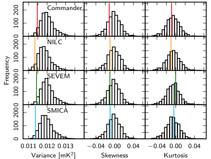
Fig. 1. Variance, skewness, and kurtosis for the four different component-separation methods — Commander (red), NILC (orange), SEVEM (green), and SMICA (blue) — compared to the distributions derived from 1000 Monte Carlo simulations.
