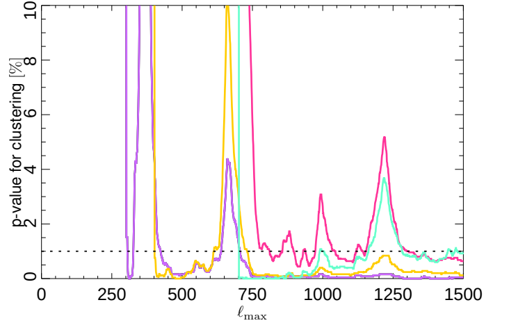
Fig. 37. Derived p -values for the angular clustering analysis as a function of \ell_{\text{max}} , determined from SMICA based on 2500 simulations. The p -values are based on the fraction of simulations with a higher Rayleigh statistic up to the given \ell_{\text{max}} than in the data. The RS here is calculated over all pairs of dipole directions where one dipole in each pair is computed in the range [\ell_{\text{lim}}, \ell_{\text{max}}] , and the other is determined in the range [2, \ell_{\text{lim}}] . The plot shows p -values for \ell_{\text{lim}} = 300 (purple), \ell_{\text{lim}} = 400 (yellow), \ell_{\text{lim}} = 500 (pink), and \ell_{\text{lim}} = 700 (cyan). The results have been marginalized over bin sizes in the range \Delta\ell = 8 to \Delta\ell = 32 .
