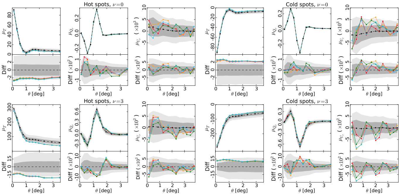
Fig. 43. Mean radial profiles of T , Q_r , and U_r in \mu\text{K} obtained for Commander (red), NILC (orange), SEVEM (green), and SMICA (blue). Each individual panel contains (top) the mean radial profiles and (bottom) the differences (denoted “Diff”) between the mean profiles of the data and those computed from the ensemble mean of the simulations. Results based on stacks around temperature hot and cold spots are shown in the left and right columns, respectively. Upper plots present results for peaks selected above the null threshold, while lower plots show the equivalent results for peak amplitudes above (hot spots) or below (cold spots) 3 times the dispersion of the temperature map. The black dots (connected by dashed lines) depict the mean profiles and the shaded regions correspond to the 1\sigma (68%) and 2\sigma (95%) error bars. The mean profiles and error bars are determined from SEVEM simulations. Note that the Diff curves for each component-separation method are computed using the corresponding ensemble average, although only the ensemble average from SEVEM is shown here.
