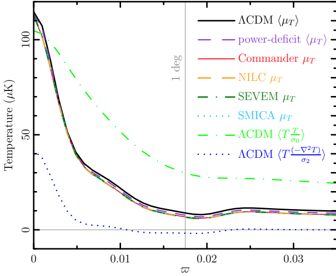
Fig. 42. Radial profile \mu_T(\omega) derived from the stacked temperature image (see Fig. 41 or 45). The denominators \sigma_0 and \sigma_2 are the theoretical rms values of CMB T and \nabla^2 T , respectively. The theoretical \langle\mu_T(\omega)\rangle is a linear combination of \langle T(\omega)(T(0)/\sigma_0)\rangle (green dash-dotted line) and \langle T(\omega)(-\nabla^2 T(0)/\sigma_2)\rangle (blue dotted line). For all four component-separated maps, the deviation of \mu_T from the ensemble mean \langle\mu_T\rangle of the fiducial model (here the Planck 2015 \Lambda CDM best fit) is consistent with cosmic variance, and can be related to the low- \ell power deficit. The example power-deficit \langle\mu_T\rangle (purple dashed line) is the theoretical prediction of \langle\mu_T\rangle if the fiducial model C_\ell s are reduced by 10% in the range 2 \leq \ell \leq 50 .
