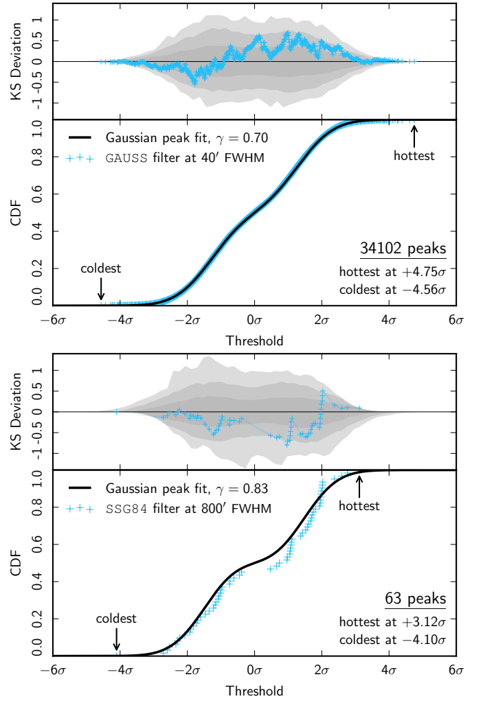
Fig. 10. Cumulative density function of the peak distribution for the SMICA CMB temperature map. The top row shows the peak CDF for maps filtered with a GAUSS kernel of 40' FWHM. The bottom row shows the corresponding peak CDF for an SSG84 kernel of 800' FWHM. The spectral shape parameter \gamma (see Eq. 27) is the best-fit value for the simulated ensemble, as indicated by the cyan circle in Fig. 11. Similar results are obtained for the other component-separation methods.
