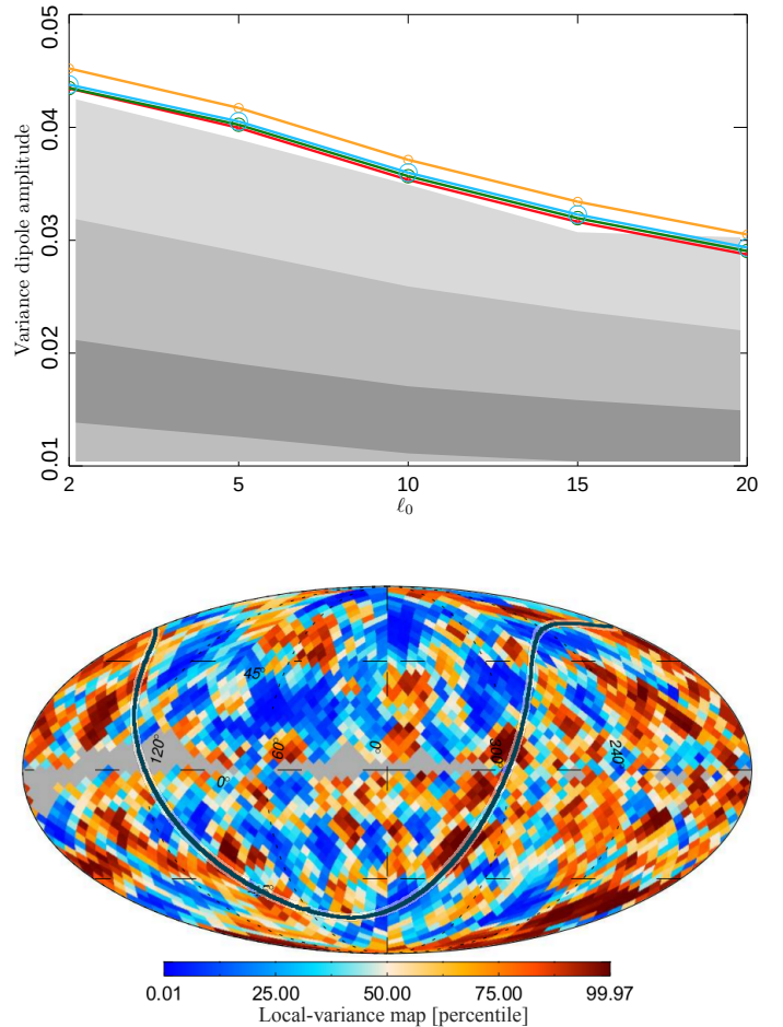
Fig. 28. Upper panel: local-variance dipole amplitude for 8^\circ discs as a function of the central multipole of the high-pass filter, \ell_0 , for the four component-separation methods, Commander (red), NILC (orange), SEVEM (green), and SMICA (blue). The grey regions, from dark to light, correspond, respectively, to 1\sigma , 2\sigma , and 3\sigma percentiles from the 1000 FFP8 simulations processed by the Commander method. Lower panel: mean-subtracted and inverse-variance-weighted local-variance map for the 8^\circ discs and for the Commander component-separation method; each pixel is given in terms of the lower- and upper-tail probability of the measured value on that pixel compared to the values from the simulations. The pixels in grey correspond to the centres of the 8^\circ discs on which the number of unmasked pixels in the full resolution map is lower than our threshold. The black curve superposed on the map indicates the boundary of the opposing hemispheres along the asymmetry axis. It is clear that the largest fraction of >95\% outliers (red pixels) lie on the positive amplitude hemisphere of the local variance dipole, while the <5\% outliers (blue pixels) are on the opposite hemisphere. The corresponding maps for NILC , SEVEM , and SMICA are very similar to the one shown here.
