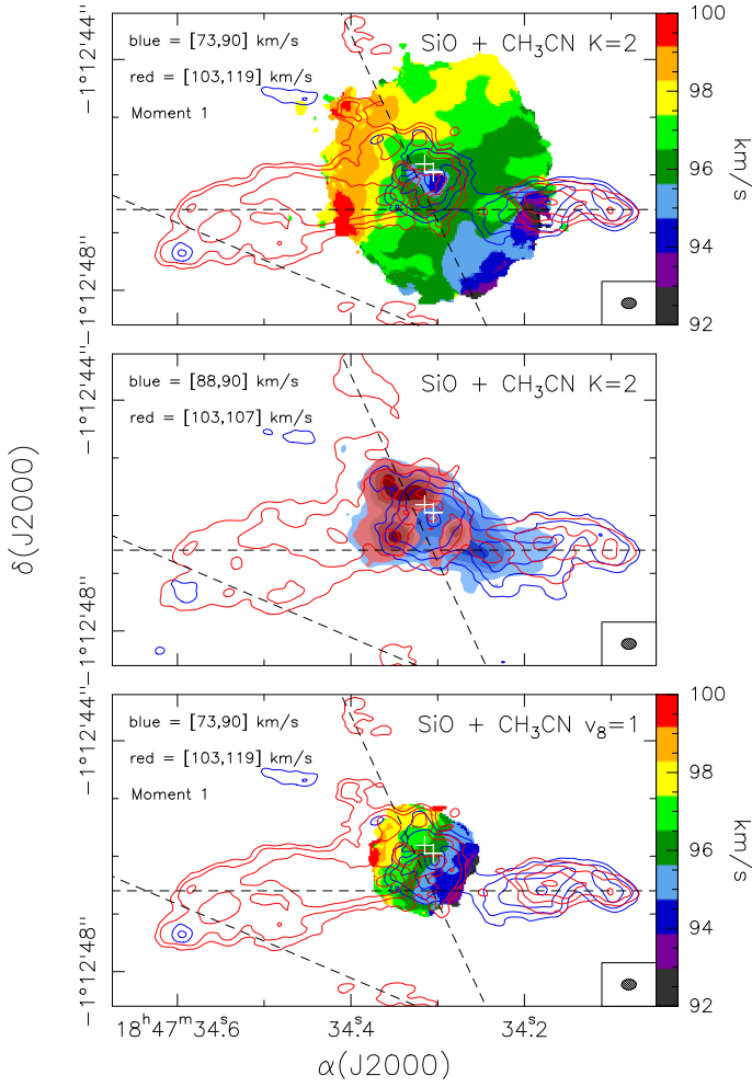
Fig. 10. Top panel: overlay of the line velocity (moment 1) map of \text{CH}_3\text{CN } K = 2 (12–11) (colors) on the \text{SiO} (5–4) blue-shifted (blue contours) and red-shifted (red contours) averaged emission. The \text{CH}_3\text{CN } K = 2 line velocity map has been computed over the velocity range (92, 100) \text{km s}^{-1} . The velocity intervals over which the \text{SiO} emission has been averaged are indicated in the upper left-hand corner. Contour levels are the same as in Fig. 5. Middle panel: overlay of the \text{CH}_3\text{CN } K = 2 (12–11) and \text{SiO} (5–4) blue-shifted and red-shifted emission averaged over the same velocity intervals, which are indicated in the upper left-hand corner. Contour and grayscale levels are 6, 18, 36, and 72 \text{mJy beam}^{-1} . Bottom panel: same as the top panel but for \text{CH}_3\text{CN } K, l = (6, -1) v_8 = 1 (12–11). The synthesized beam is shown in the lower right-hand corner. The white crosses indicate the positions of the two compact free-free continuum sources detected by Cesaroni et al. (2010). The black dashed lines indicate the direction of the three possible outflows.
