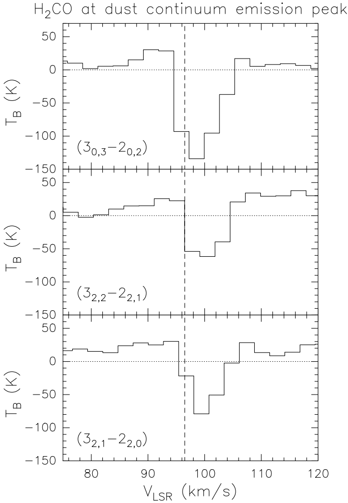
Fig. 4. \text{H}_2\text{CO} ( 3_{0,3}-2_{0,2} ), ( 3_{2,2}-2_{2,1} ), and ( 3_{2,1}-2_{2,0} ) spectra at the dust continuum emission peak. The vertical dashed line indicates the systemic LSR velocity of 96.5 \text{ km s}^{-1} .
