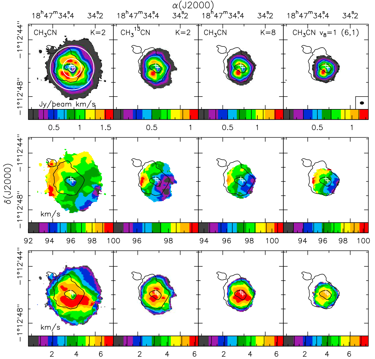
Fig. A.2. Top panels: overlay of the 217 GHz continuum emission (black contours) on the integrated intensity (moment 0) map (colors) of \text{CH}_3\text{CN } K=2 , \text{CH}_3^{13}\text{CN } K=2 , \text{CH}_3\text{CN } K=8 , and \text{CH}_3\text{CN } K, l = (6, 1) v_8 = 1 (12–11). The contours correspond to the 5\sigma and 50% levels. The concentric white circles in the first panel have radii of 0''.22 , 0''.66 , and 1''.54 , (see Sects. 4.1 and 4.2). Middle panels: line velocity (moment 1) maps for the same molecular species. Bottom panels: velocity dispersion (moment 2) maps for the same species. The white crosses indicate the positions of the two compact free-free continuum sources detected by Cesaroni et al. (2010). The synthesized beam is shown in the lower right-hand corner of the top right panel.
