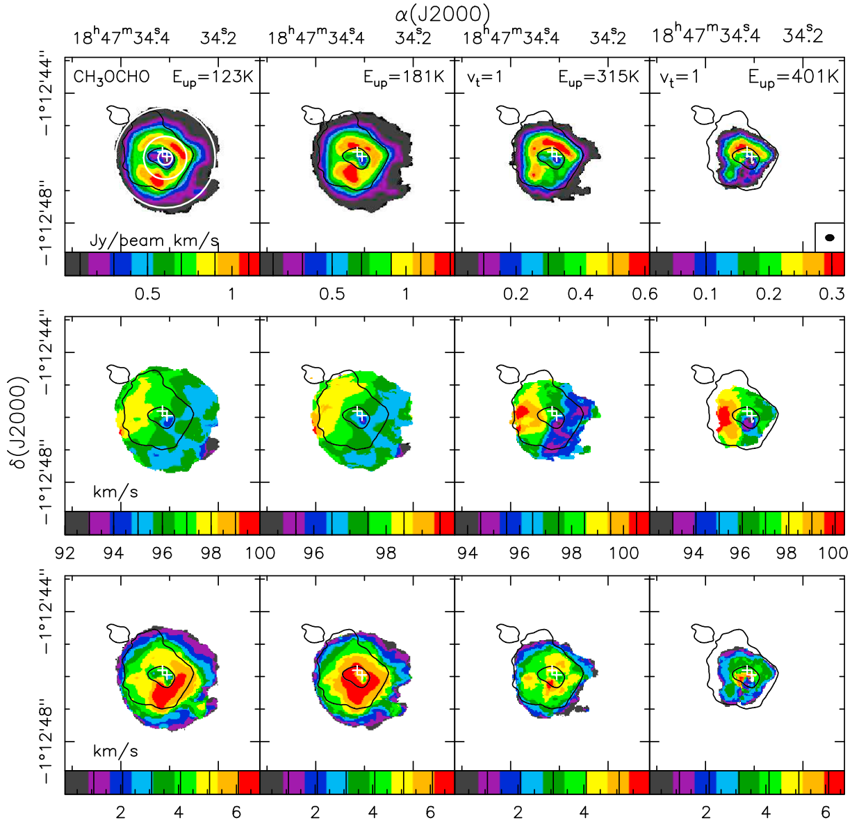
Fig. A.3. Same as Fig. A.2 for CH 3 OCHO (19 4,16 -18 4,15 )A, (18 11,7 -17 11,6 )A, (20 2,18 -19 2,17 )A v t = 1, and (18 13,6 -17 13,5 )E v t = 1. The upper level energies E up of each transition are indicated in the upper right-hand corner of the top panels.
