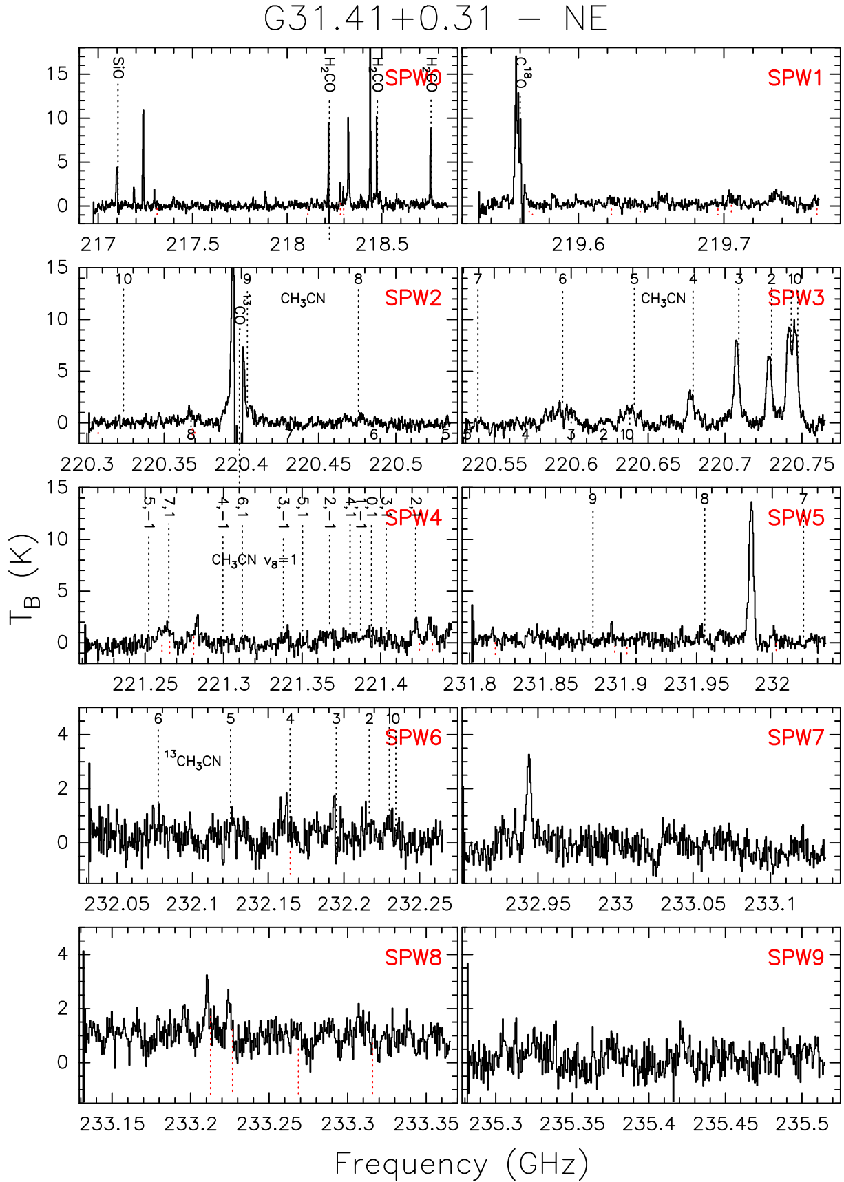
Fig. A.1. Same as Fig. 2 for the NE source.
