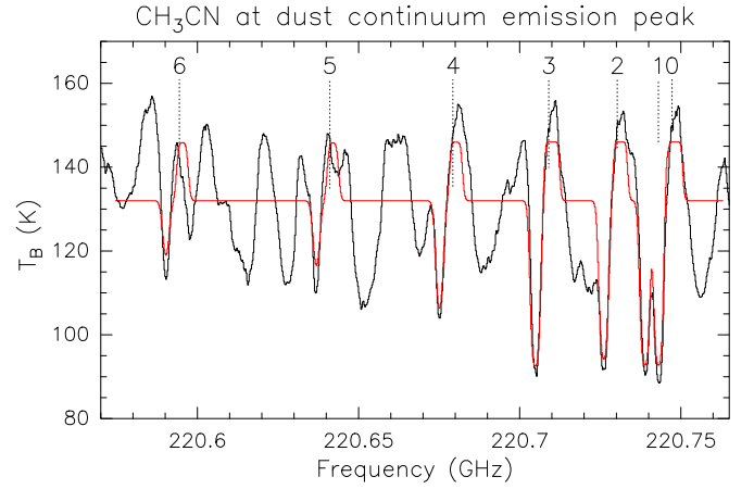
Fig. 12. Spectrum obtained at the dust continuum emission peak of the G31 Main core (black) and best fit to the \text{CH}_3\text{CN}(12-11) K = 0 to 6 transitions (red). The spectrum has been modeled with different components: i) a background layer with homogeneous intensity to describe the dust continuum core, ii) a core layer to describe the emission, and iii) a foreground layer located in front of the core component to describe the absorption (see Sect. 5.2.2). We note that the other emission and absorption lines not fitted correspond to other species.
