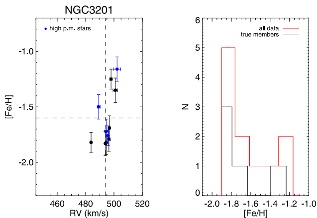
Figure 7. Left-hand panel: RV–abundance plot for RV candidate members which fall within the tidal radius of NGC 3201. The dashed lines indicate the nominal RV and [\text{Fe}/\text{H}] for the cluster reported in the literature. The blue dots are stars with large proper motions with respect to the measured proper motion for the cluster. Right-hand panel: The metallicity distribution function for all RV candidate members which fall within the tidal radius (in red) and for those which also have proper motion measurements consistent with that of the cluster (black line).
