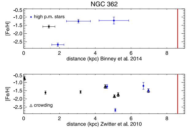
Figure 18. Distance versus [\text{Fe}/\text{H}] for the members of NGC 362. In the top panel are plotted the distances derived in Binney et al. (2014); however, there are only four stars with this information. In the bottom panel the distances from Zwitter et al. (2010) are shown. Blue dots are stars with a large proper motion; triangles indicate stars affected by crowding. The vertical red line indicates the distance of the cluster from Harris (1996)–2010 edition.
