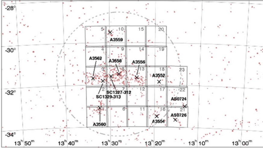
Fig. 27.1 The 23 1 \text{ deg}^2 VST fields mapping the ShaSS region. Red dots indicate the supercluster members in the range V_h = 11,300\text{--}17,000 \text{ km s}^{-1} taken from literature. The size of the dots are proportional to the K -band flux. Black crosses show the cluster centres. The 10 Mpc radius dotted circle encloses the supercluster region believed to be dynamically bound. The SSCC corresponds to fields #3,8,13. The positions of all structures present in the plotted area are indicated
