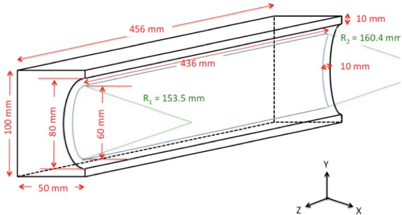
Figure 2: geometric parameters of the BEaTriX paraboloidal mirror. In the BEaTriX setup, the microfocus source will be placed on the minimum diameter side, at approx. 4741 mm from the beginning of the optically-finished part, measured along the axis. In the PANTER setup, the full X-ray illumination comes from the max. diameter side, and will involve the central 400 mm \times 60 mm area.
