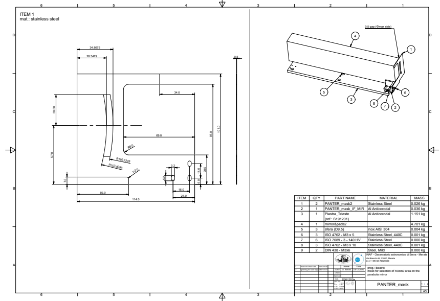
Figure 7: drawing of the slit placed in front of the mirror and interface plate.
