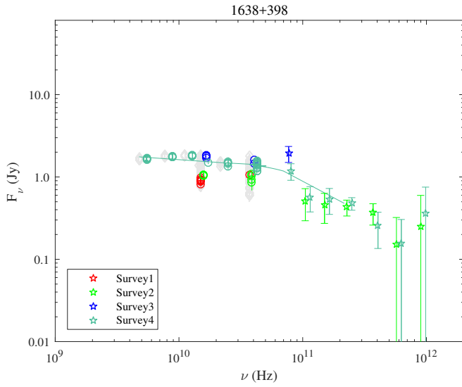
Fig. A.71. 1638+398.
