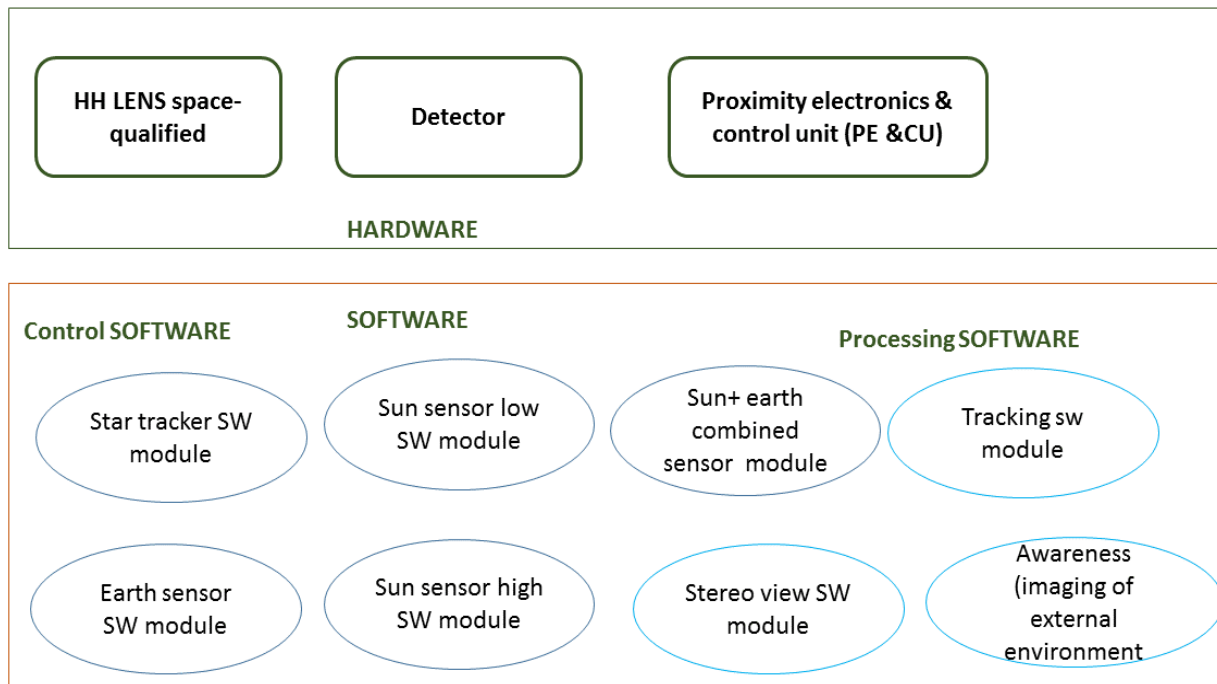
Figure 9: POLIFEMO components.
