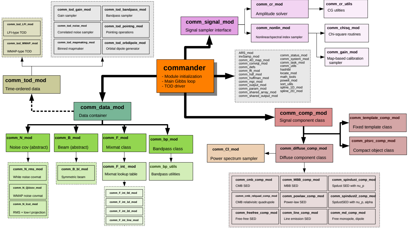
Fig. 2. Overview of the Commander source code. The main program is called commander.f90 and is indicated by the orange box in the center. All other boxes represent individual modules, except the gray box to the right, which summarizes various utility modules.
