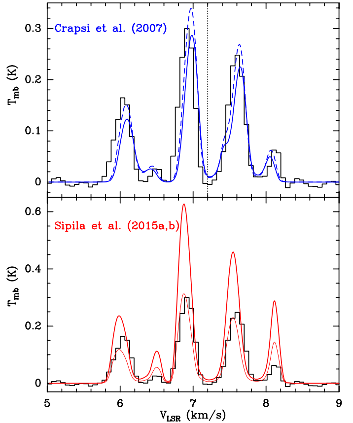
Fig. 4. MOLLIE radiative transfer results using the \text{o-NH}_3 fractional abundance profiles from Fig. 3, overlapped with the observed spectrum: (top) blue solid and dashed curves refer to the Crapsi et al. (2007) profiles, assuming an ortho-to-para \text{NH}_3 ratio of 0.7 and 1.0, respectively. (Bottom) The red thick curve refers to the Sipilä et al. (2015a,b) profile; the red thin curve is the same as the thick red curve, but divided by 2.
