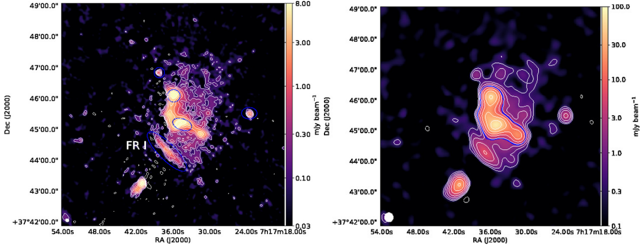
Figure 4. Left panel: GMRT image at 608 MHz at high resolution ( 6.3'' \times 5.6'' ). The rms noise is 30\mu\text{Jy/beam} . Right panel: GMRT image at 608 MHz at low resolution ( 18.3'' \times 17.4'' ). The noise is 0.1 mJy/beam. Blue circles and ellipses indicate the sources embedded in the diffuse emission, that have been masked. In both panels, contours start at 4\sigma and are spaced by a factor 2. Contour at -4\sigma are dashed. The restoring beams are shown in the bottom-left corner of the two panels.
