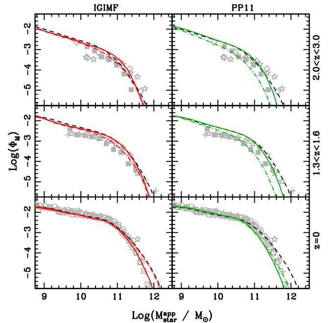
Figure 2. Redshift evolution of the GSMF. In each panel, the black long-dashed line refers to the predictions of the H16F model; the solid lines to the GSMF as a function of M_*^{\text{app}} and the dot-dashed lines to the GSMF as a function of the intrinsic galaxy stellar mass M_* . Grey points show a collection of observational measurements as in Fontanot et al. (2009, see detailed references herein).
