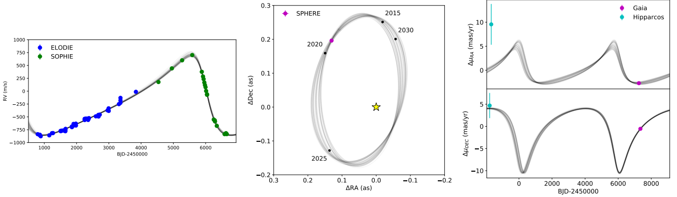
Fig. 2. Sample of 50 model orbits fitted on the HD 72946B data (colored points) from RV (left), imaging (middle), and astrometry (right). Middle panel: yellow star marks the location of the primary star, and the black dots show the median predicted position for given epochs.
