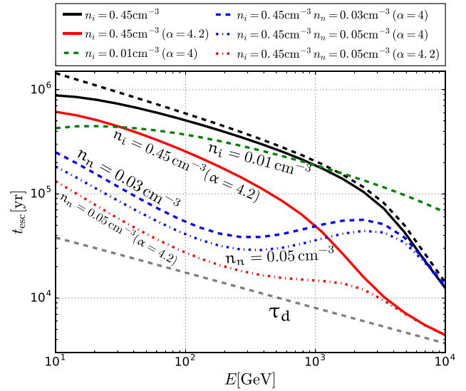
Figure 2. CR escape time t_{esc} (see the text for exact definition) as a function of particle energy for four different types of ISM: (1) no neutrals and n_i = 0.45 \text{ cm}^{-3} (black solid line); (2) n_n = 0.03 \text{ cm}^{-3} and n_i = 0.45 \text{ cm}^{-3} (blue dashed line); (3) n_n = 0.05 \text{ cm}^{-3} and n_i = 0.45 \text{ cm}^{-3} (blue dot-dashed line); (4) no neutrals and n_i = 0.01 \text{ cm}^{-3} (green dashed line). The black dashed line represents case (1) but without the advection term in both equations (1) and (10). The solid red line represents case (1), but with a steeper injection spectrum, \alpha = 4.2 ; analogously, the dot-dashed red line corresponds to case (3) with \alpha = 4.2 . For all other curves, the slope is \alpha = 4 . The grey dashed line represents the standard diffusion time \tau_d = L_c^2/D_g = 8.3 \times 10^4 (E_{\text{GeV}})^{-1/3} yr.
