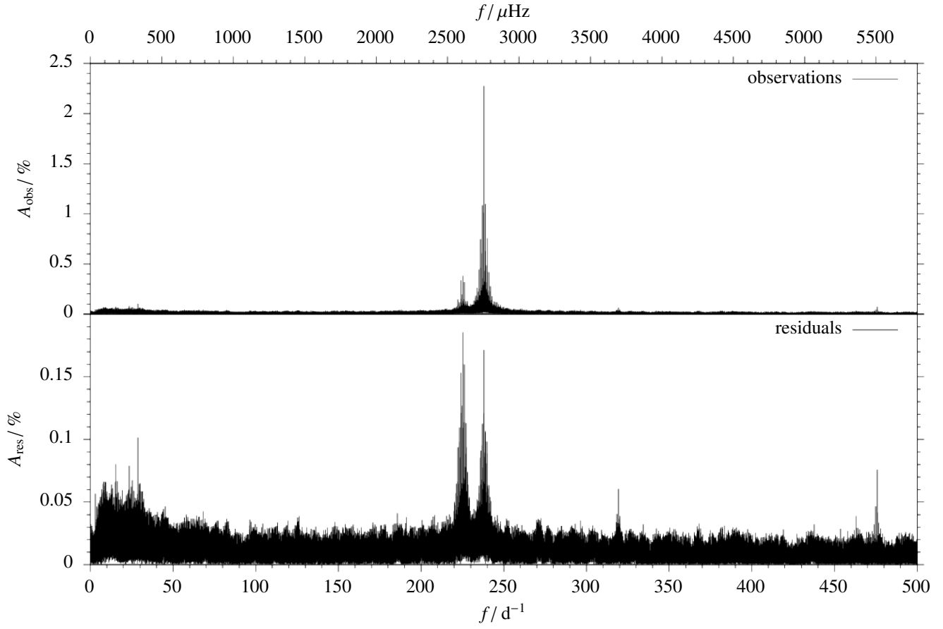
Fig. B.1: Amplitude spectrum of DW Lyn. The upper panel shows the observations A_{\text{obs}} . The lower panel shows the residuals A_{\text{res}} after subtracting the light curve models from the observations.
