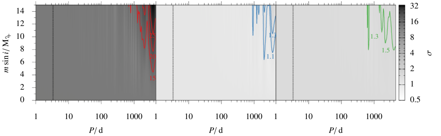
(c) QQ Vir. Contour lines for f_1 are placed at 15, 20, and 25 \sigma (left panel), for f_2 at 1.1 and 1.3 \sigma (middle panel), and for f_3 at 1.3 and 1.5 \sigma (right panel), as indicated by their labels.
