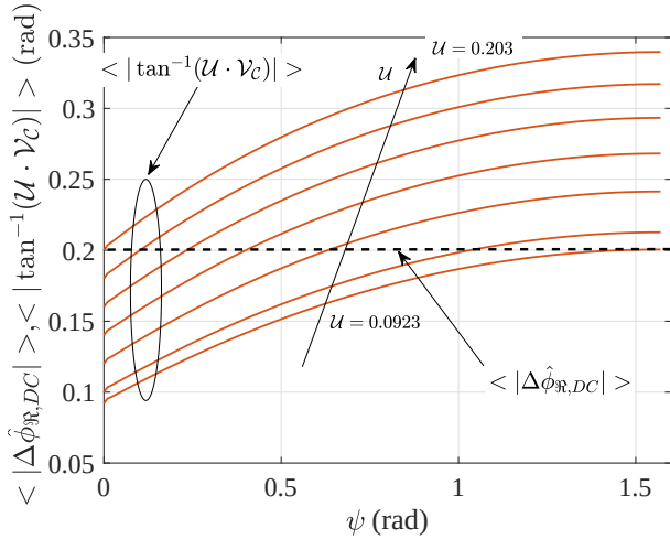
Fig. 10: Dependence of the function \langle |\Delta\phi_{\mathcal{R},DC}| \rangle on the variable \psi fixing different values of \mathcal{U} . The intersections of those curves with the measured value \langle |\Delta\hat{\phi}_{\mathcal{R},DC}| \rangle restrict the possible solution to a small interval of \mathcal{U} .
