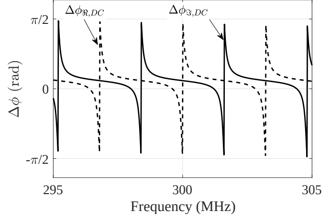
Fig. 2: Example of theoretical behaviors of \Delta\phi_{\Re,DC} = \tan^{-1} [\mathcal{U} \cdot \mathcal{V}_C] and \Delta\phi_{\Im,DC} = \tan^{-1} [\mathcal{U} \cdot \mathcal{V}_S] for different values of M , \psi . Note that the functions exhibit fast variations with respect to f_{RF} even in the short frequency interval considered. See text for details.
