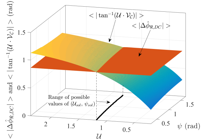
Fig. 12: 3D plot of the function \langle |\Delta\phi_{\mathcal{R},DC}| \rangle and of the plane \langle |\Delta\hat{\phi}_{\mathcal{R},DC}| \rangle . The intersection produces possible couples of solution (\mathcal{U}_{sol}, \psi_{sol}) .
