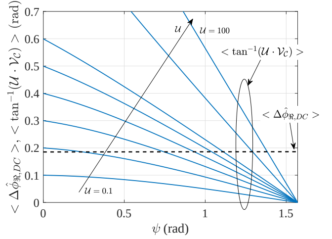
Fig. 11: Dependence of the function \langle \Delta\phi_{\mathcal{R},DC} \rangle on the variable \psi fixing different values of \mathcal{U} . In this case the range of possible values of \mathcal{U} is larger, making the resolution of the problem difficult.
