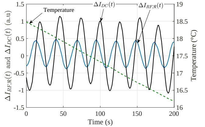
Fig. 5: Typical measurement in the time domain of \Delta I_{DC}(t) and \Delta I_{RF,\mathcal{R}}(t) . The value of the modulating frequency is f_{RF} = 300 MHz. The phase shift between the two fluctuating behaviors is clearly visible. In this case it is \Delta\phi_{\mathcal{R},DC} \simeq -0.075 rad.
