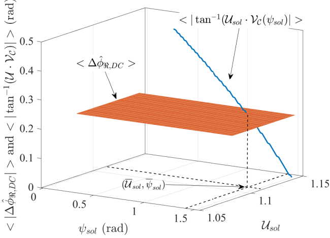
Fig. 13: 3D plot of the function \langle \Delta\phi_{R,DC} \rangle computed in the values founded in the first step (U_{sol}, \psi_{sol}) . The intersection with the plane corresponding to \langle \Delta\phi_{R,DC} \rangle gives the final solution.
