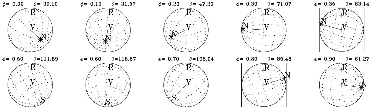
Fig. 8. Changes of the geometry of CU Vir as a function of the rotational phase. The point V at the center of the star is the intersection of the stellar surface with the line of view; the point R close to the top is the rotational pole; the points denoted with N and S represent the North and South magnetic poles; the arc V-N subtends the angle \theta_M . \phi and \theta_M are indicated in each panel. The main peaks are visible when the star is oriented as in the two framed panels at \phi \approx 0.35 (peak a) and at \phi \approx 0.80 (peak d).
