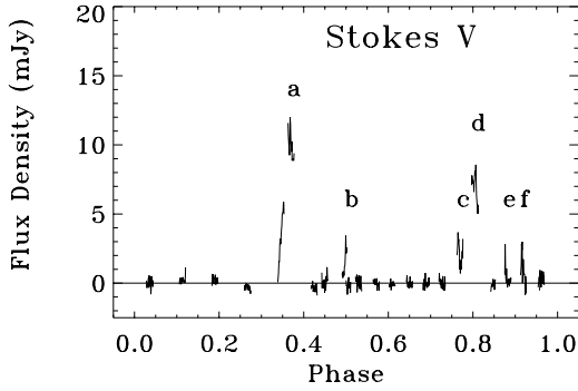
Fig. 5. Stokes parameter V versus rotational phase in the 3 days of observation. No polarization is seen outside the peaks denoted with the letters from a to f. The higher fluxes (a and d) are visible when the magnetic axis is perpendicular to the line of sight.
