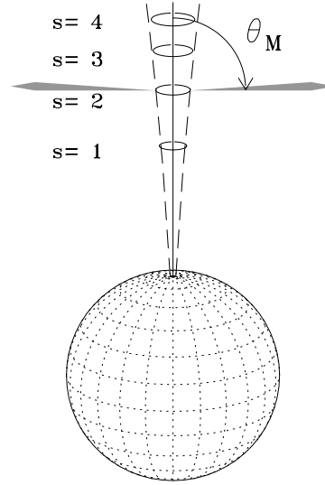
Fig. 11. Proposed picture for the emission of the main peaks. Accelerated in the current sheets and flowing back to the surface following the magnetic field lines (dashed lines from the pole) electrons are reflected by magnetic mirrors close to the star; they develop a loss cone anisotropy and emit cyclotron maser when going outward; the location of the possible region of the maser emission at 1.4 GHz are the circular rings centered around the axis of the dipole (vertical straight line); each ring is marked with the corresponding harmonic number s . The shaded areas represent the escaping radiation if generated, for example, at harmonic s=2 . The angle \theta_M is also shown.
