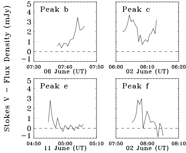
Fig. 12. Secondary peaks. See text for details.
