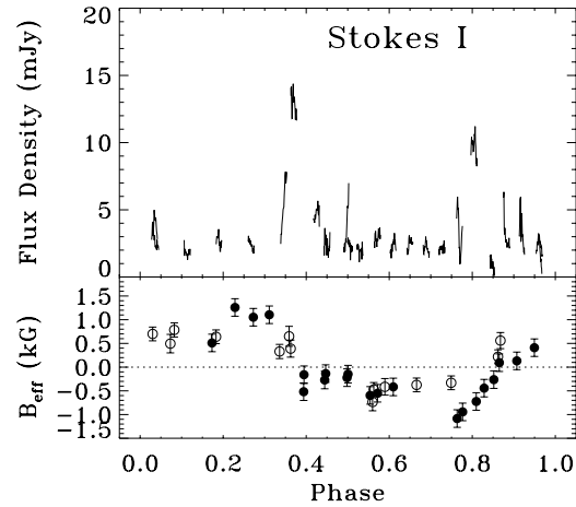
Fig. 4. Upper panel: 1.4 GHz emission from CU Vir; Lower panel: Longitudinal magnetic field measurements from Borra & Landstreet (1980) and from Pyper et al. (1998) (open and filled circles respectively) as a function of the rotational phase. 1.4 GHz radiation maxima correspond approximately with the null magnetic field.
