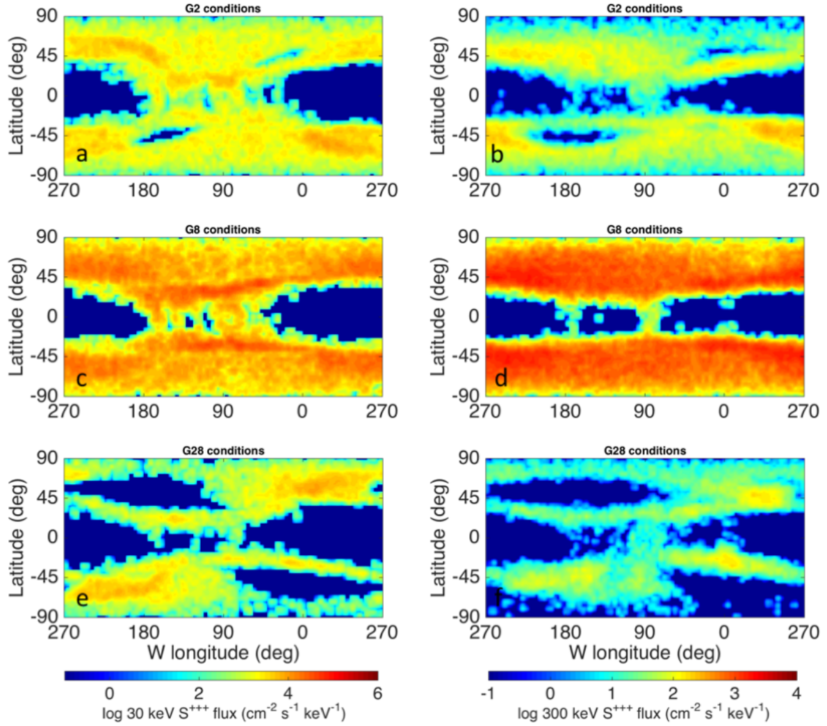
Figure 6: 30 keV S^{+++} (panels (a), (c), and (e)) and 300 keV S^{+++} (panels (b), (d), and (f)) precipitation to Ganymede's surface for different configurations of the moon's magnetic field with respect to JPS. Panels (a) and (b) correspond to magnetic field conditions similar to those during the Galileo G2 flyby (Ganymede above the centre of JPS), panels (c) and (d) to those during the Galileo G8 flyby (Ganymede near the centre of JPS), panels (e) and (f) to those during the Galileo G28 flyby (Ganymede below the centre of JPS). The W longitude system has been used meaning the leading hemisphere is at long \sim 90^\circ and long \sim 0^\circ is at the Jupiter-facing hemisphere apex.
