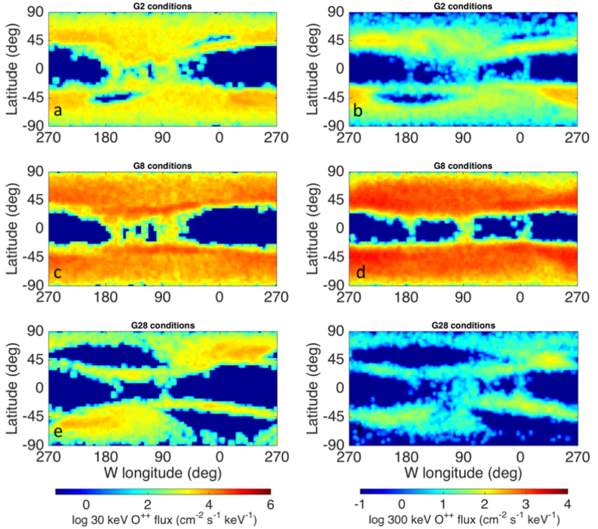
Figure 5: 30 keV O^{++} (panels (a), (c), and (e)) and 300 keV O^{++} (panels (b), (d), and (f)) precipitation to Ganymede's surface for different configurations of the moon's magnetic field with respect to JPS. Panels (a) and (b) correspond to magnetic field conditions similar to those during the Galileo G2 flyby (Ganymede above the centre of JPS), panels (c) and (d) to those during the Galileo G8 flyby (Ganymede near the centre of JPS), panels (e) and (f) to those during the Galileo G28 flyby (Ganymede below the centre of JPS). The W longitude system has been used meaning the leading hemisphere is at long \sim 90^\circ and long \sim 0^\circ is at the Jupiter-facing hemisphere apex.
