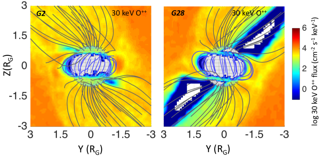
Figure 7: Circulation maps of O^{++} at initial energy equal to 30 keV in science case (i) (Ganymede above the centre of JPS; left panel) and (iii) (Ganymede below the centre of JPS; right panel). The GPhiO coordinates have been used: X is along the ambient flow direction (and Ganymede's orbital motion), Z is along the Jupiter's spin axis, and Y points toward Jupiter (in units of Ganymede's radii).
