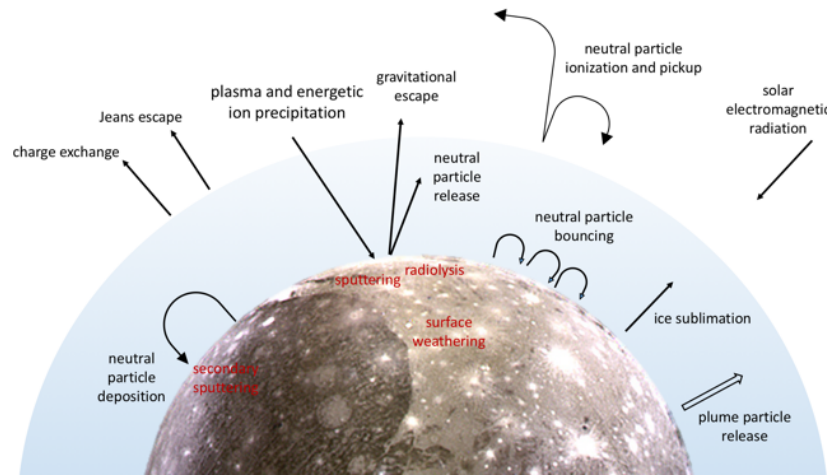
68 69 Figure 1: Source and loss mechanisms for the exosphere of Ganymede. The moon's environment is 70 strongly coupled with the Jovian magnetosphere through a series of dynamical processes that 71 contribute to the overall energy exchange between the two systems. Ganymede image credit: 72 NASA/JPL/DLR.
