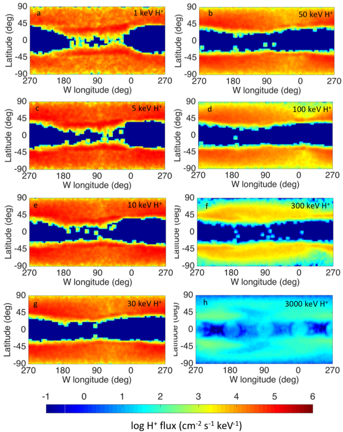
303 Figure 3: H^+ precipitation maps in science case (ii) (Ganymede is near the centre of JPS) 304 corresponding to different initial energies. The W longitude system has been used meaning the 305 leading hemisphere is at long \sim 90^\circ and long \sim 0^\circ is at the Jupiter-facing hemisphere apex.
