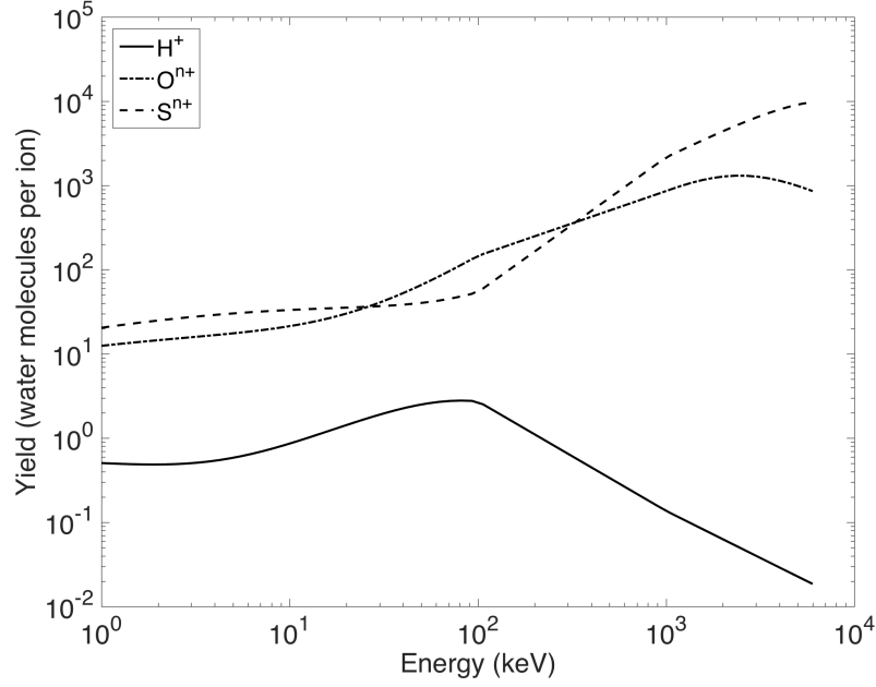
Figure 9: Water release yield due to the precipitation of H^+ , O^{n+} , S^{n+} in the energy range 1 keV – 7 MeV. Yield values are from Teolis et al. (2017).
